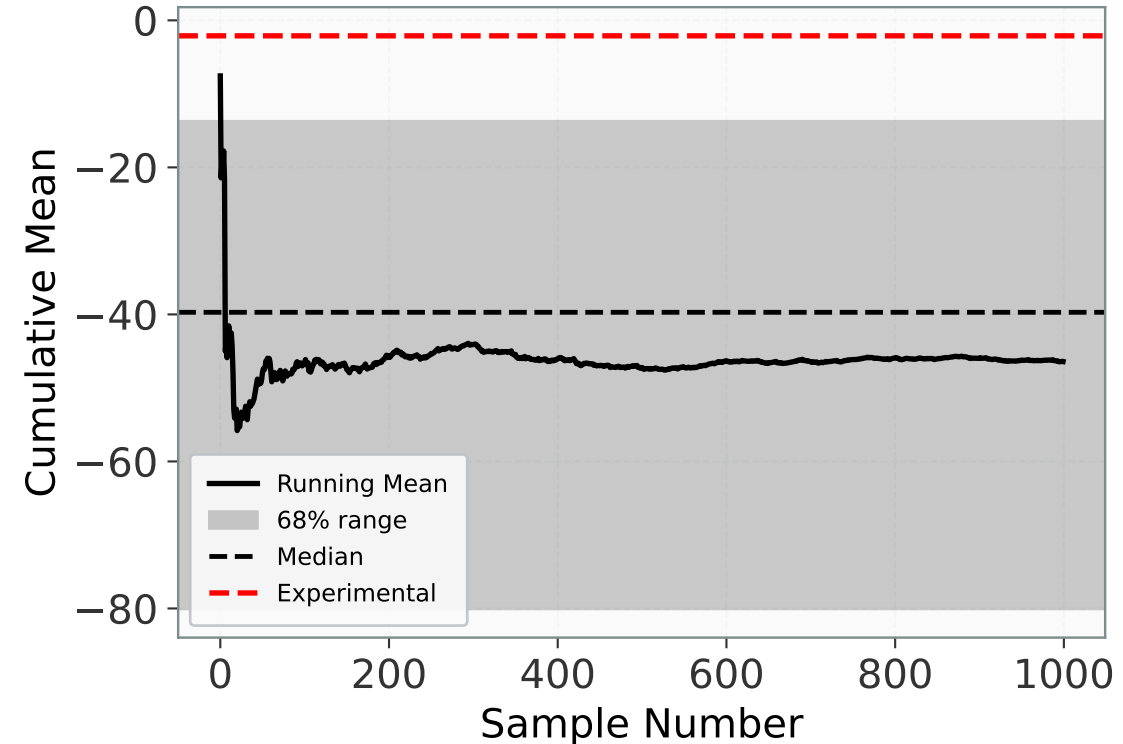
Convergence: \xi_{180,60}
