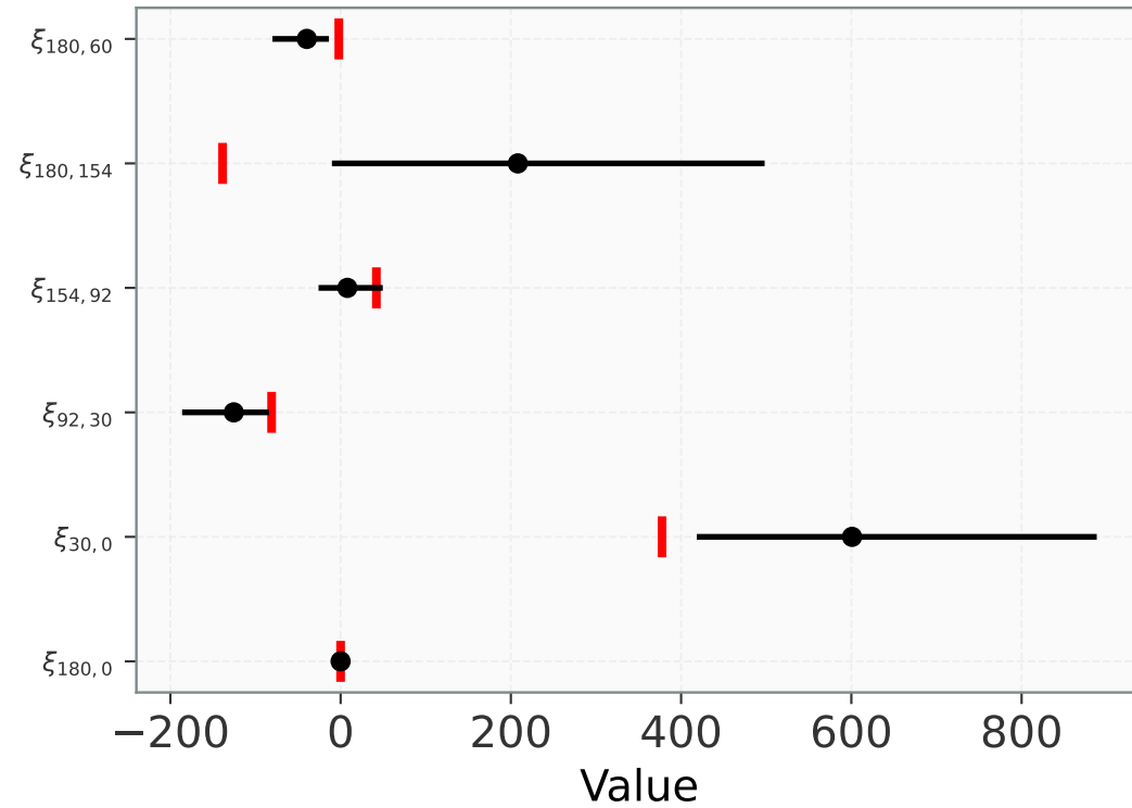
68% Credible Intervals
