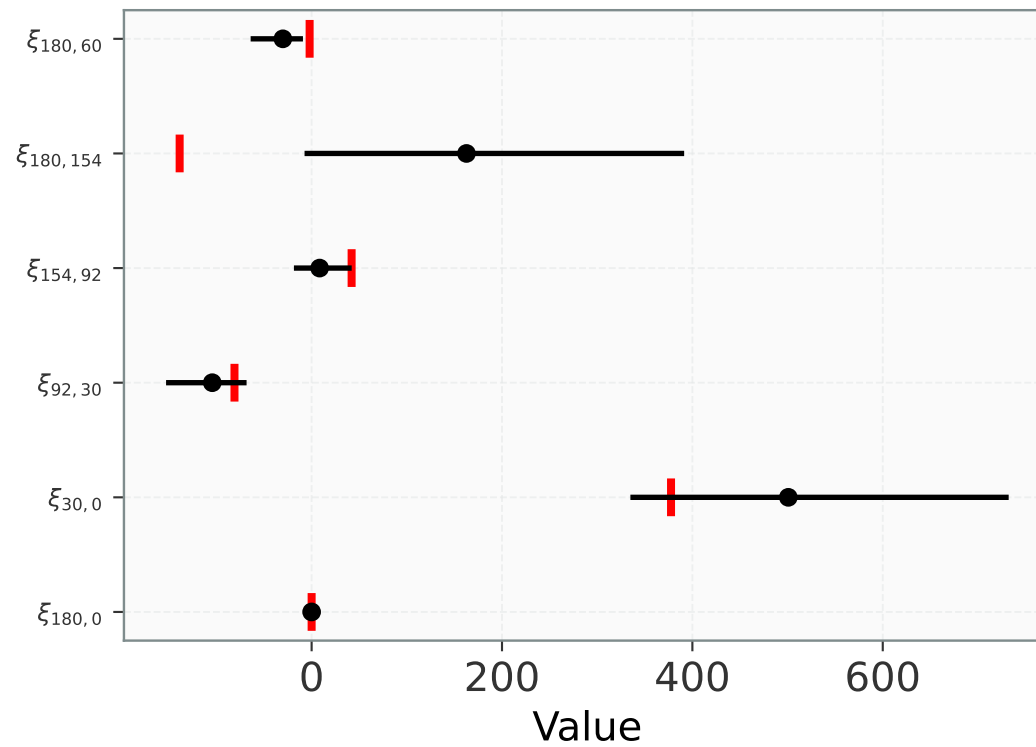
68% Credible Intervals
