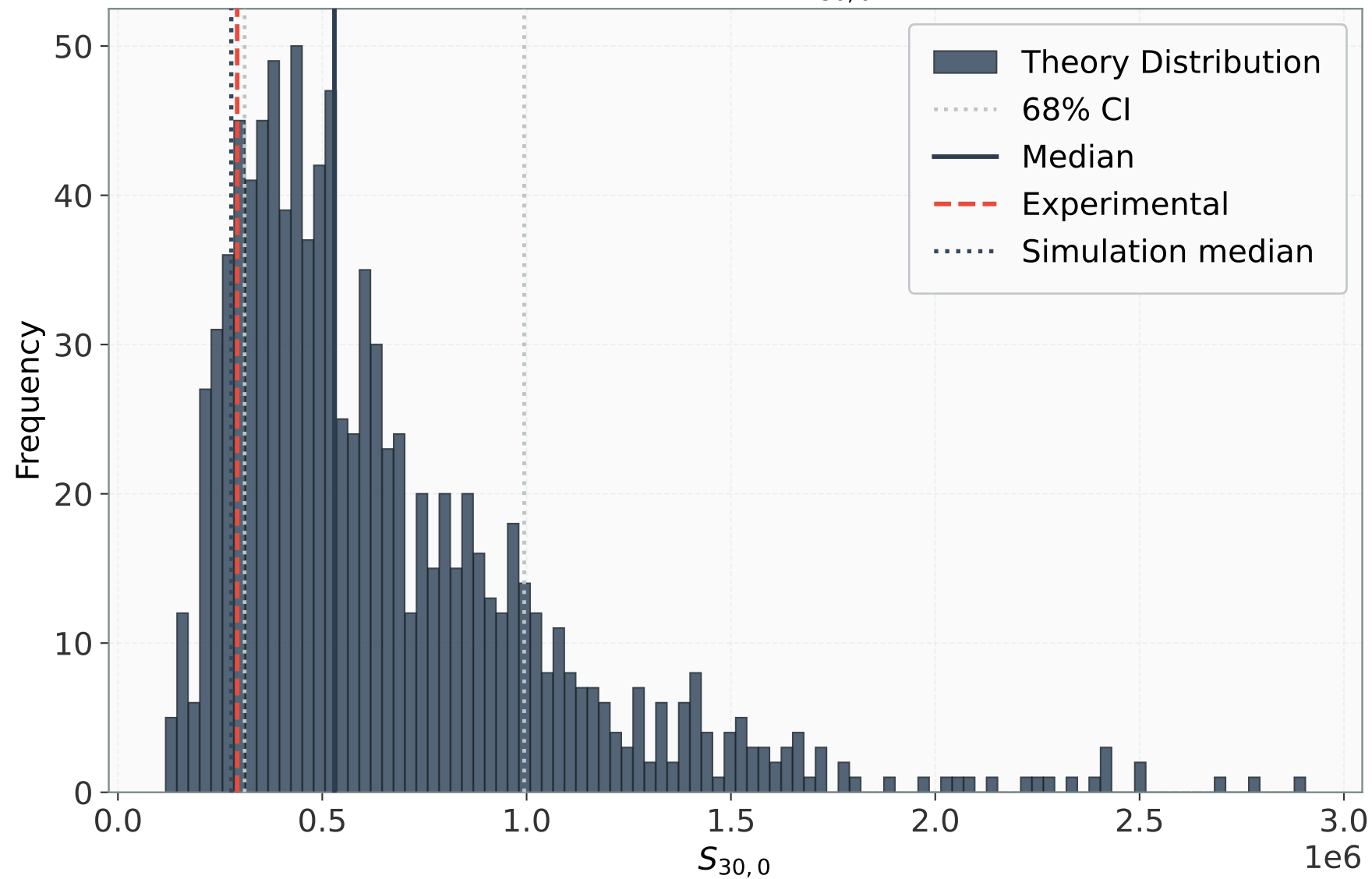
Distribution: S_{30,0}
