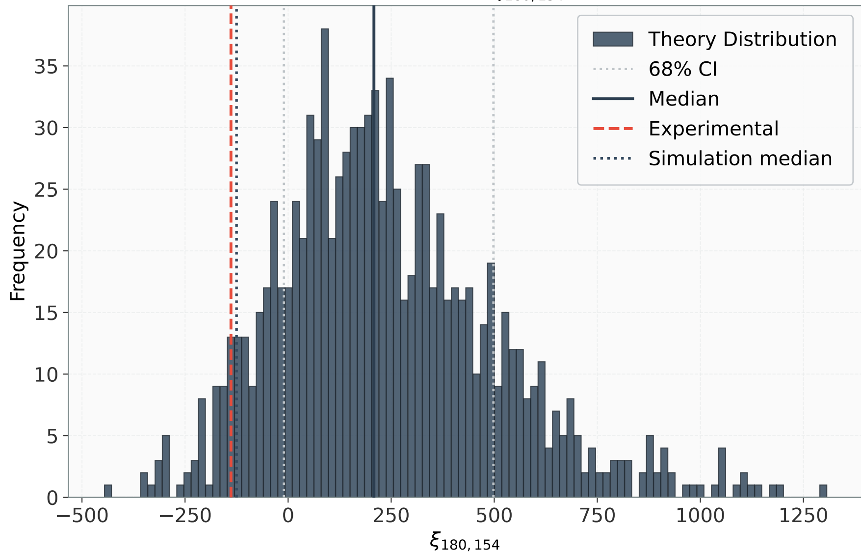
Distribution: \xi_{180,154}
