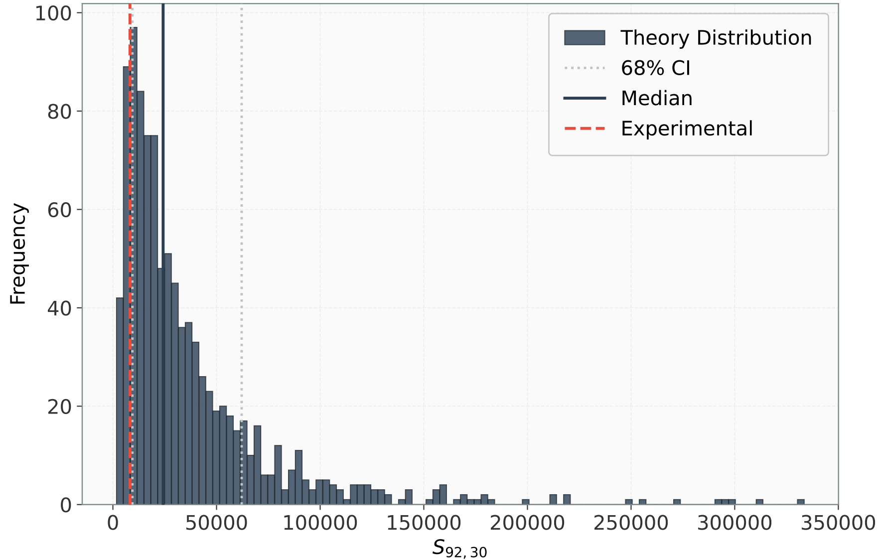
Distribution: S_{92,30}
