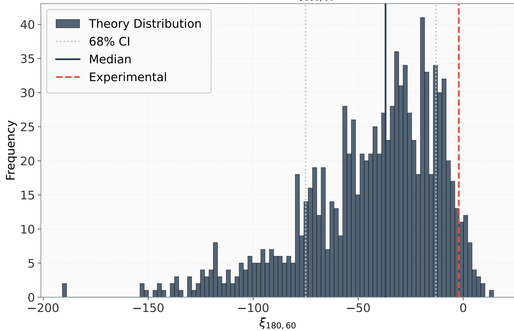
Distribution: \xi_{180,60}
