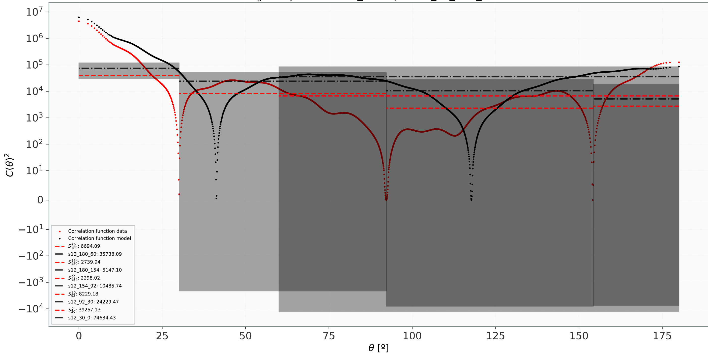
S_a^b analysis for base_CamSpecHM_TT_lowl_lowE
