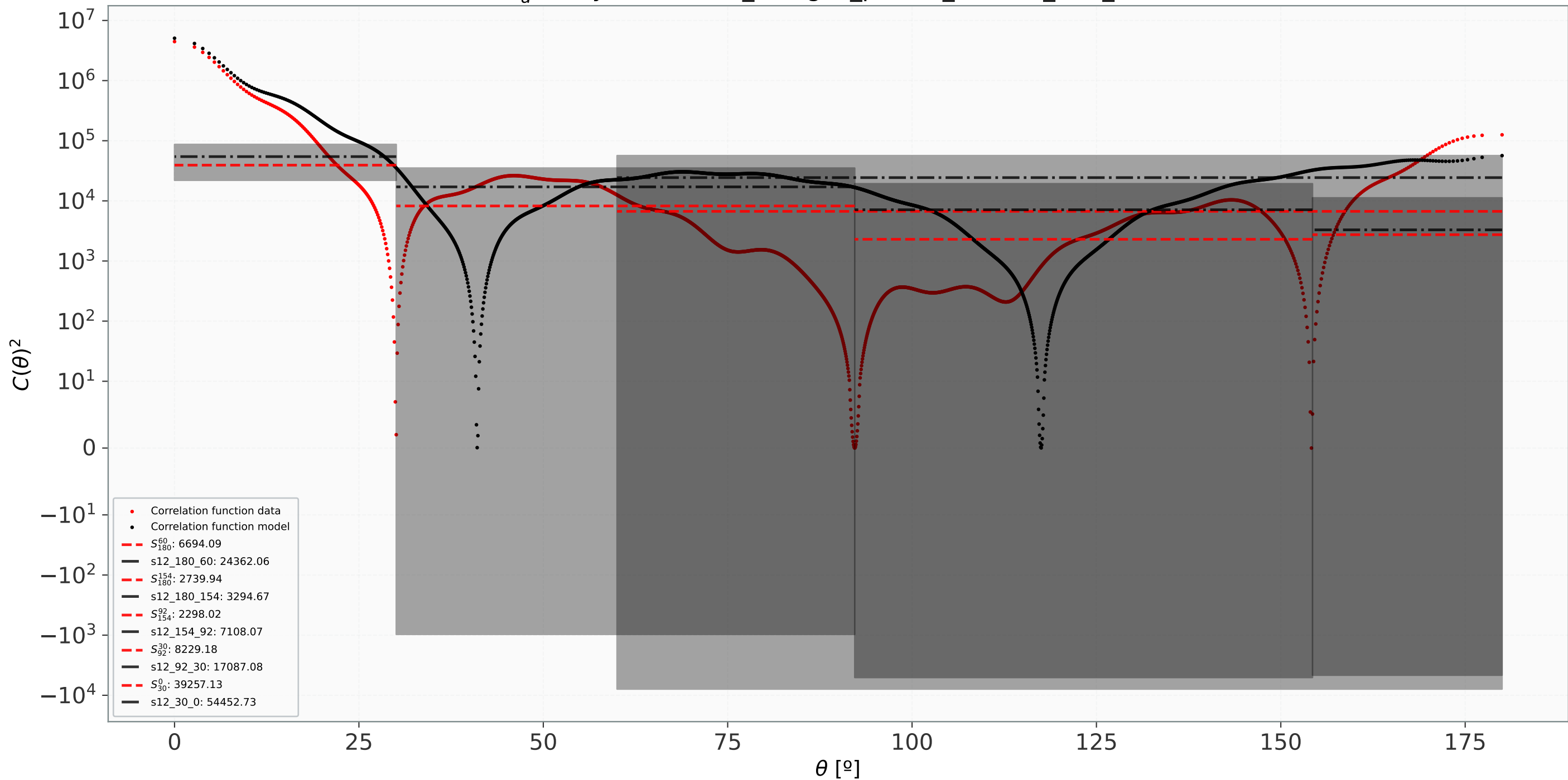
S_a^b analysis for base_omegak_plikHM_TTTEEE_lowl_lowE
