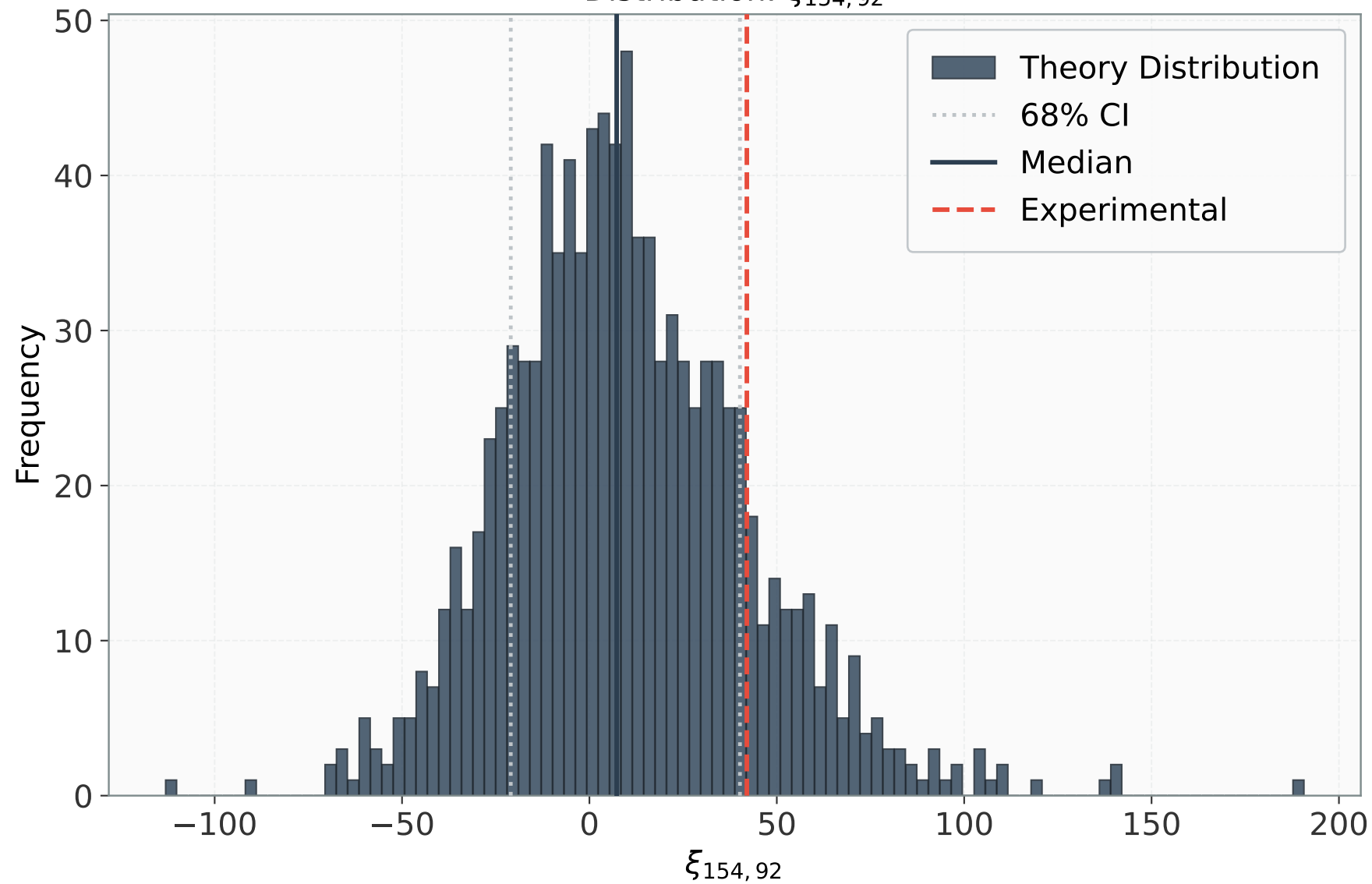
Distribution: \xi_{154, 92}
