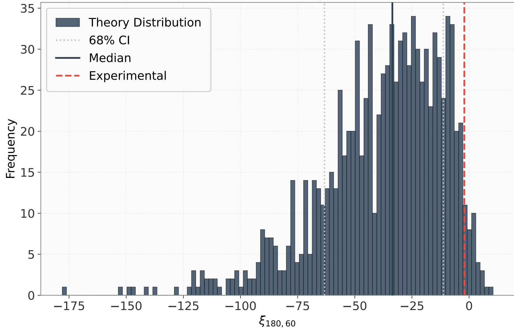
Distribution: \xi_{180,60}
