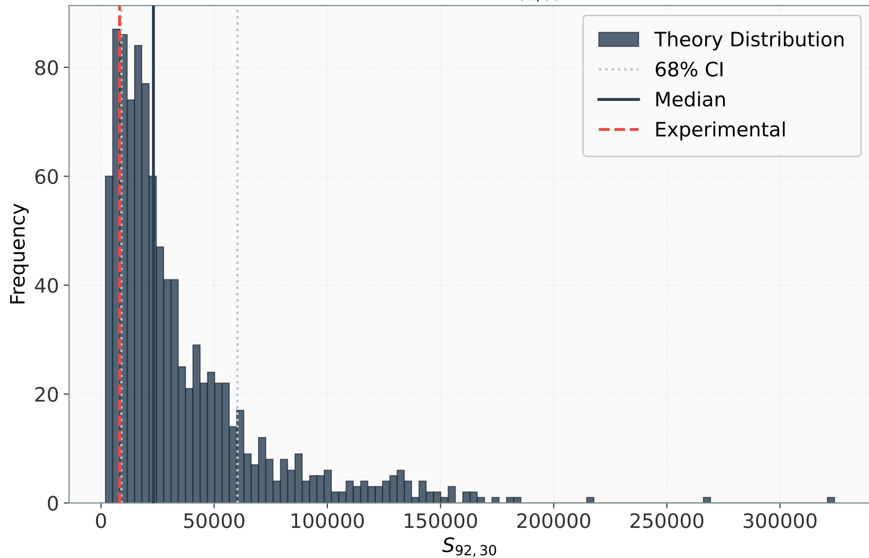
Distribution: S_{92,30}
