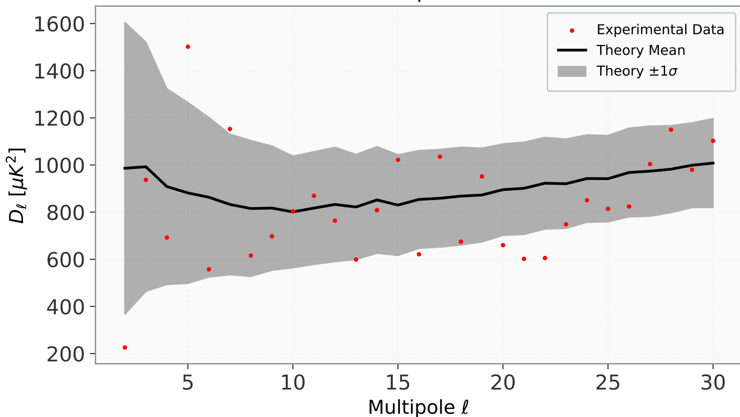
Power Spectrum
