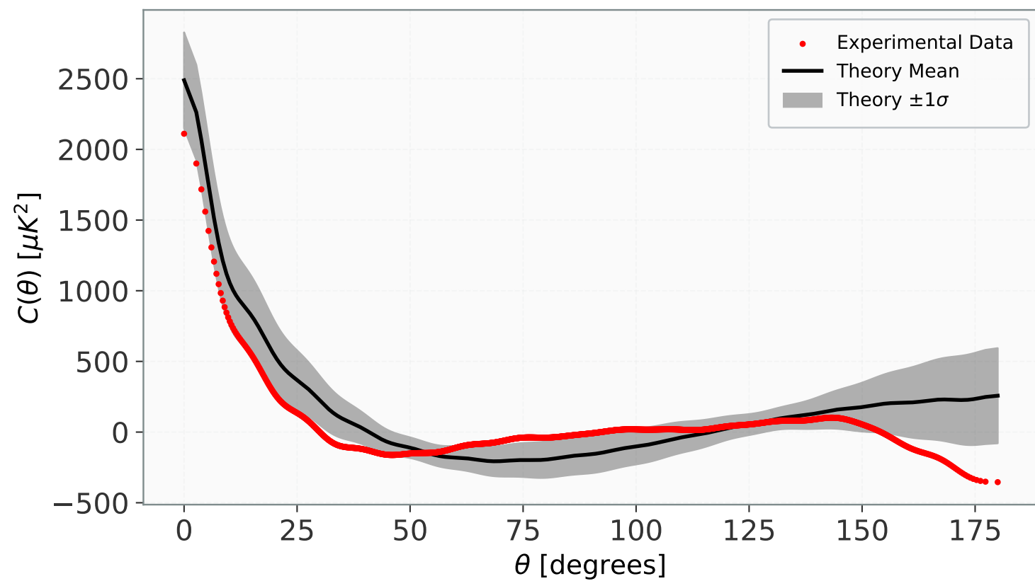
Correlation Function
