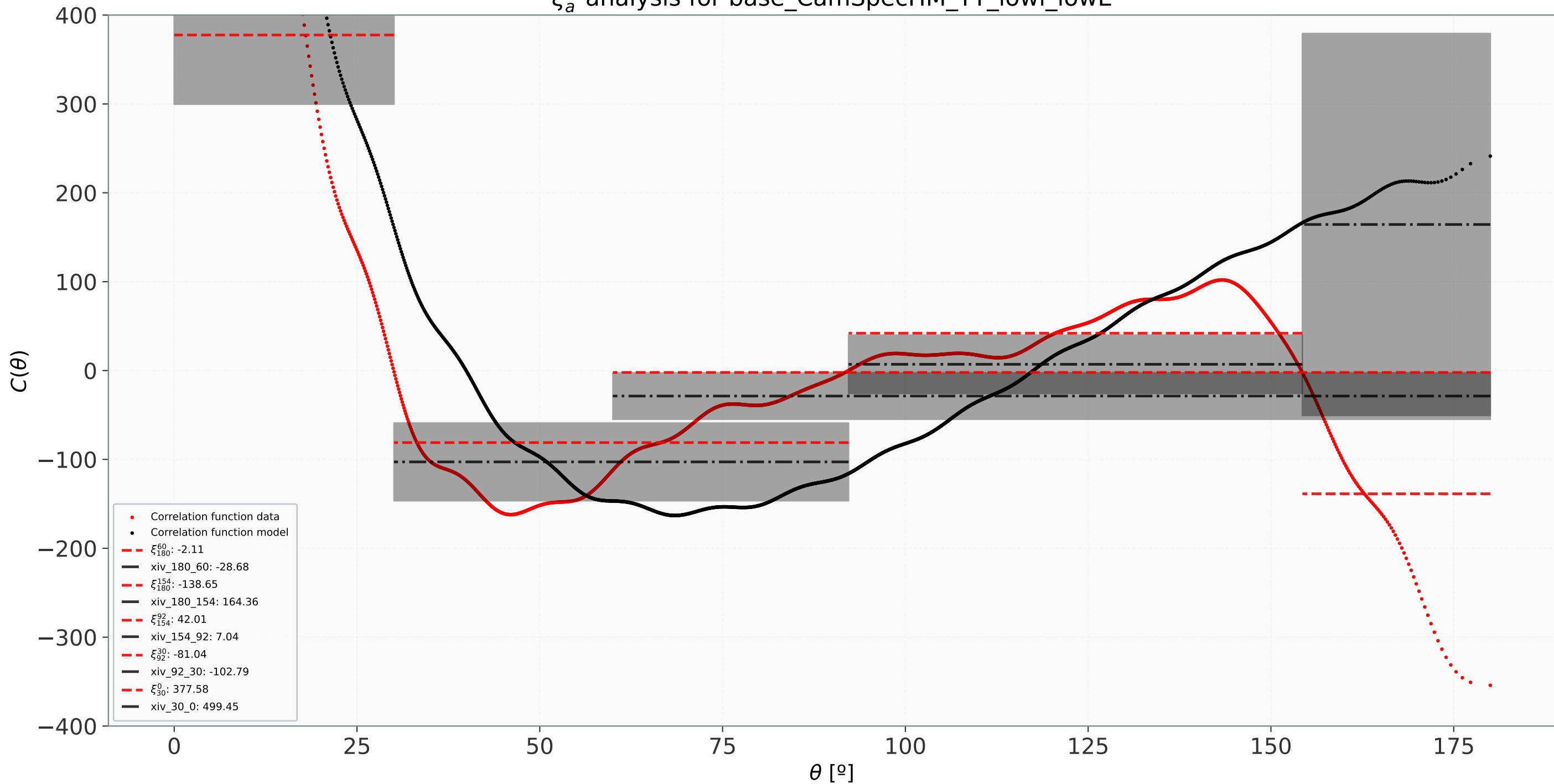
\xi_a^b analysis for base_CamSpecHM_TT_lowl_lowE
