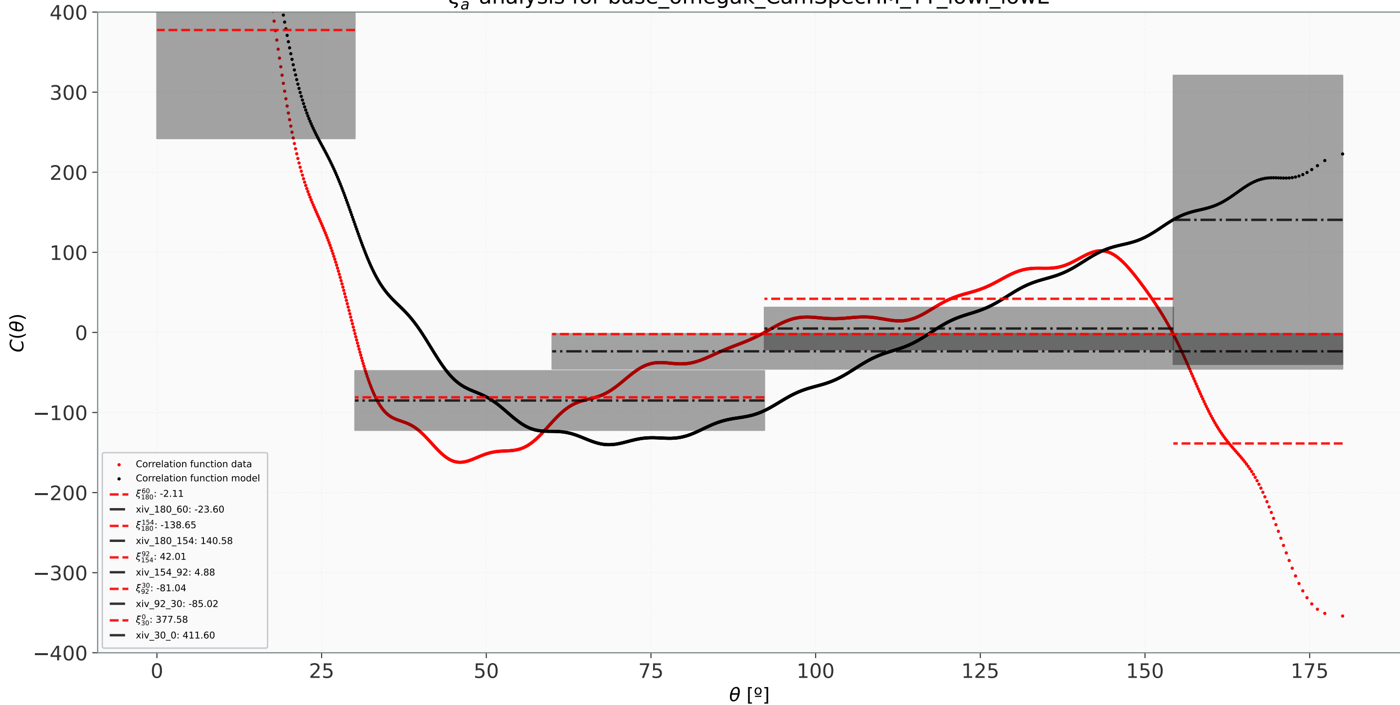
\xi_a^b analysis for base_omegak_CamSpecHM_TT_lowl_lowE
