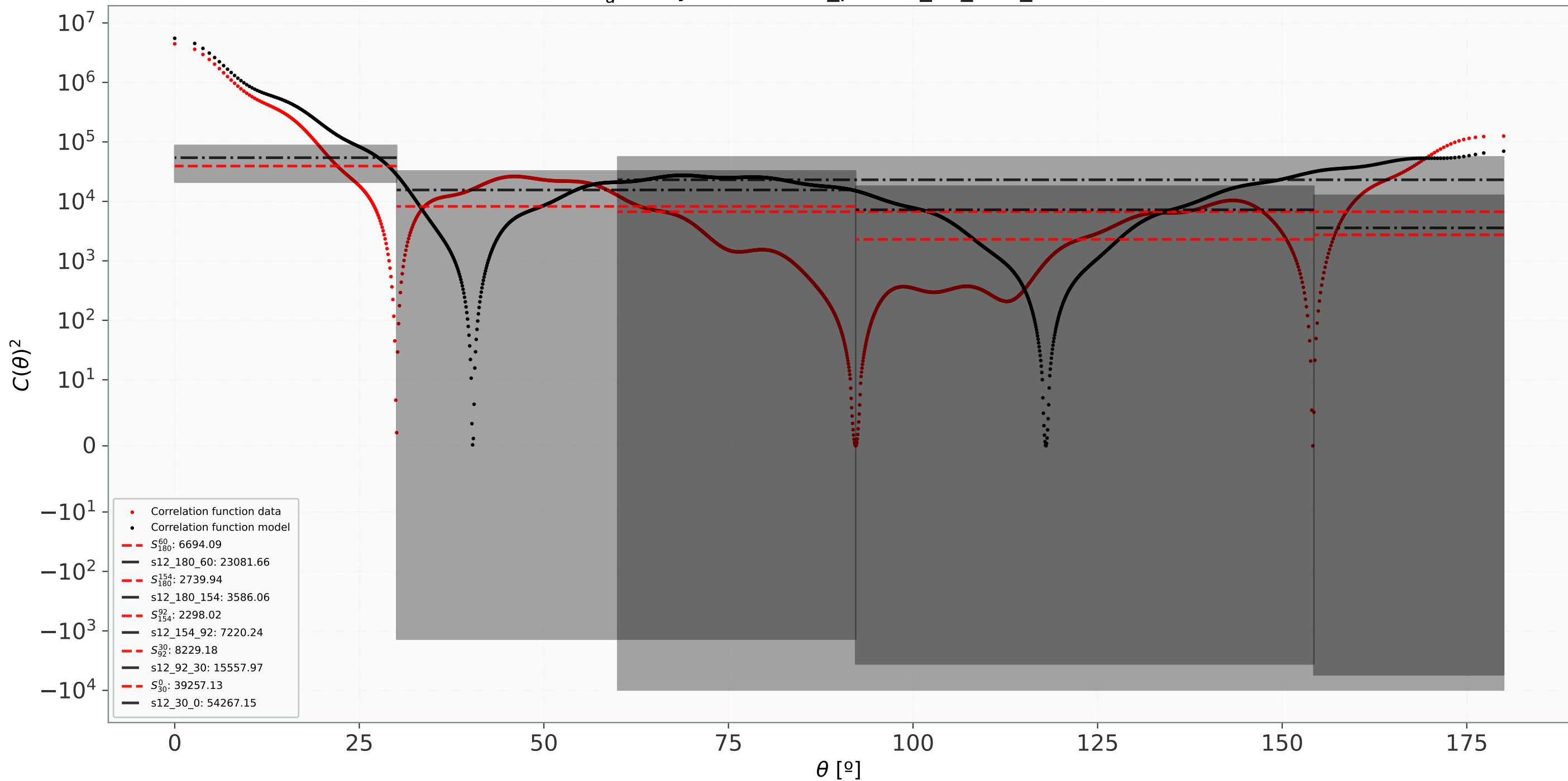
S_a^b analysis for base_plikHM_TT_lowl_lowE
