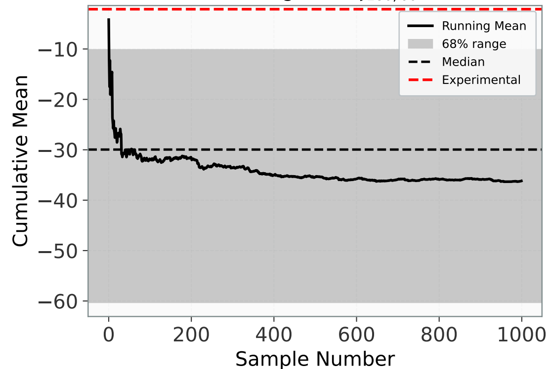
Convergence: \xi_{180,60}
