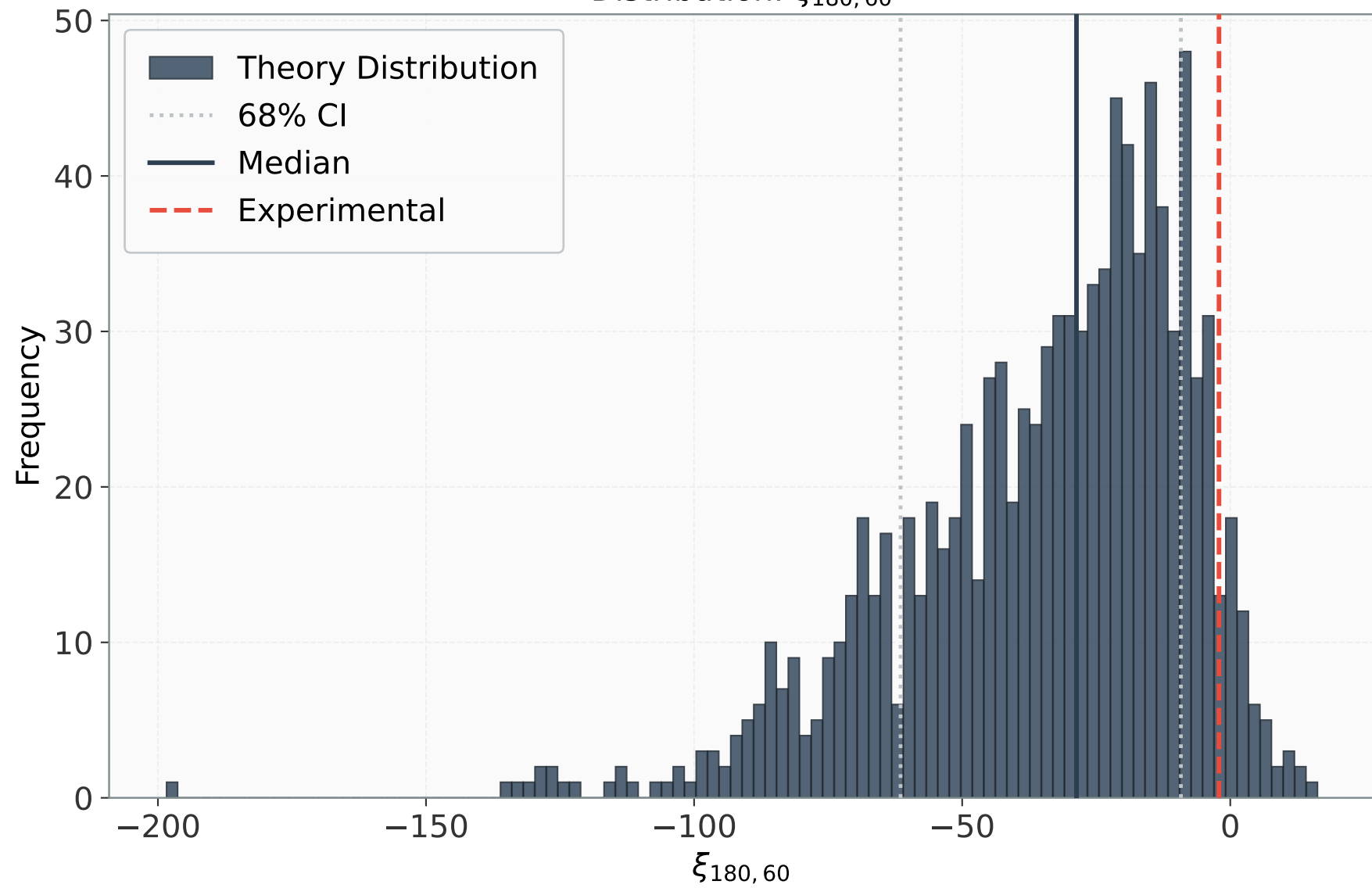
Distribution: \xi_{180,60}
