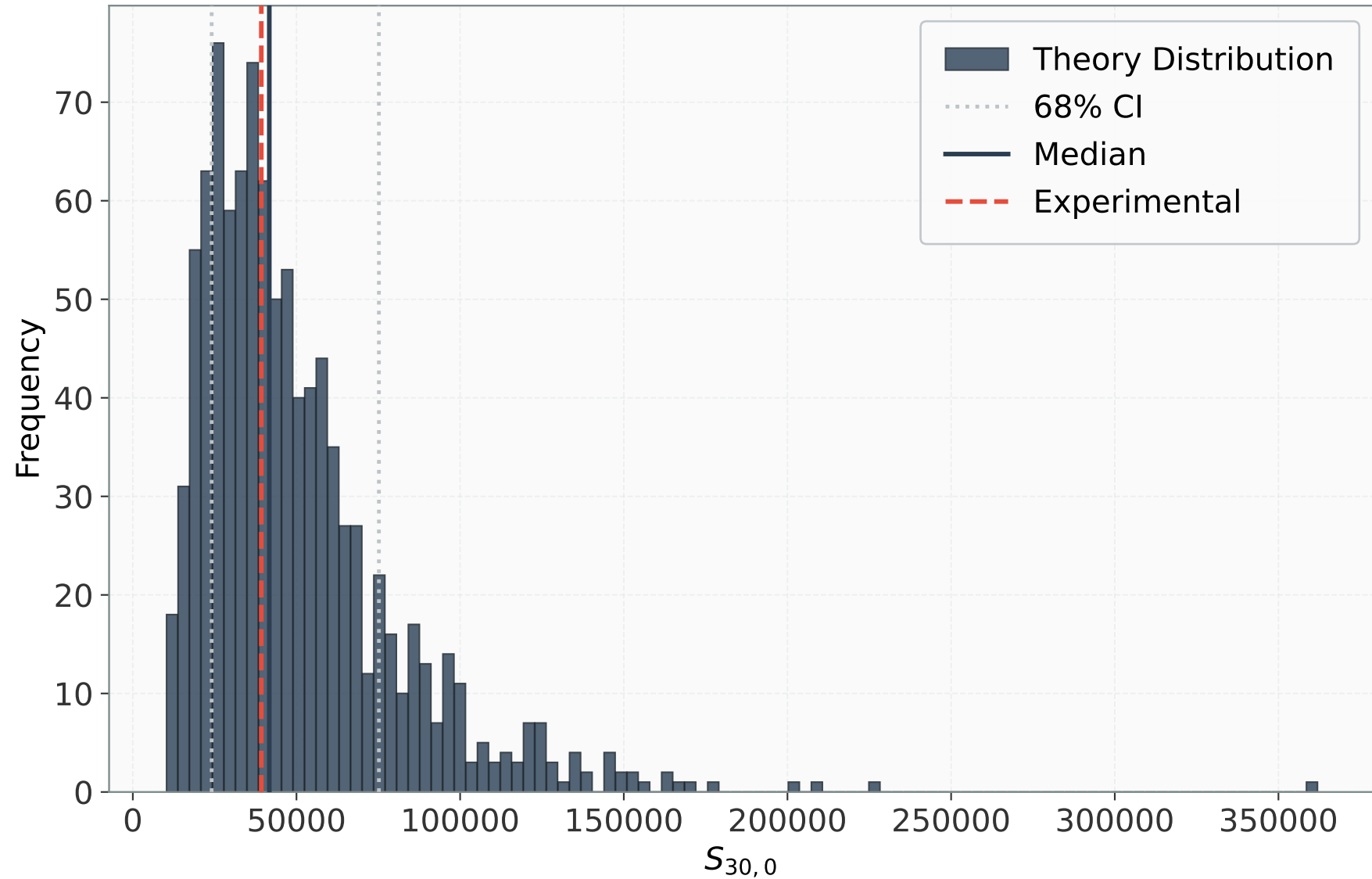
Distribution: S_{30,0}
