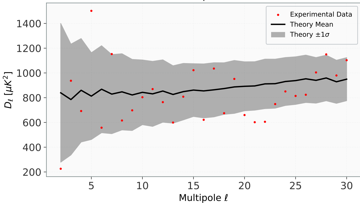
Power Spectrum
