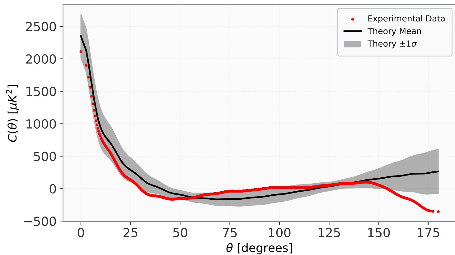
Correlation Function
