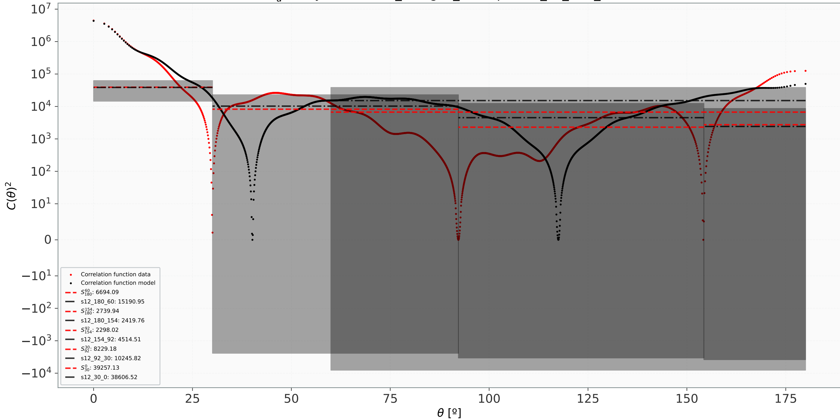
S_a^b analysis for base_omegak_CamSpecHM_TT_lowl_lowE
