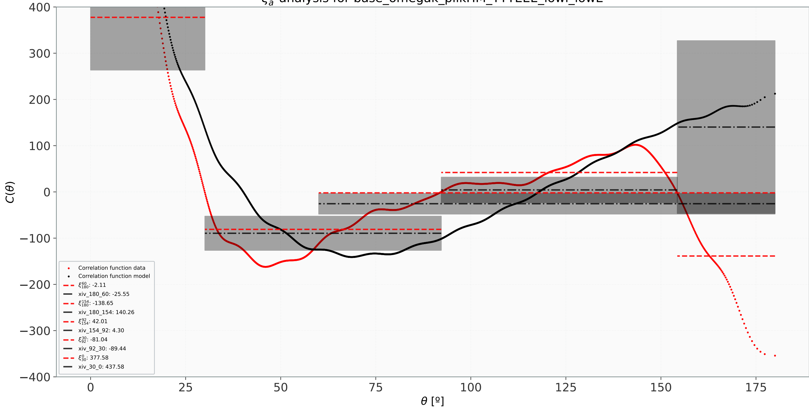
\xi_a^b analysis for base_omegak_plikHM_TTTEEE_lowl_lowE
