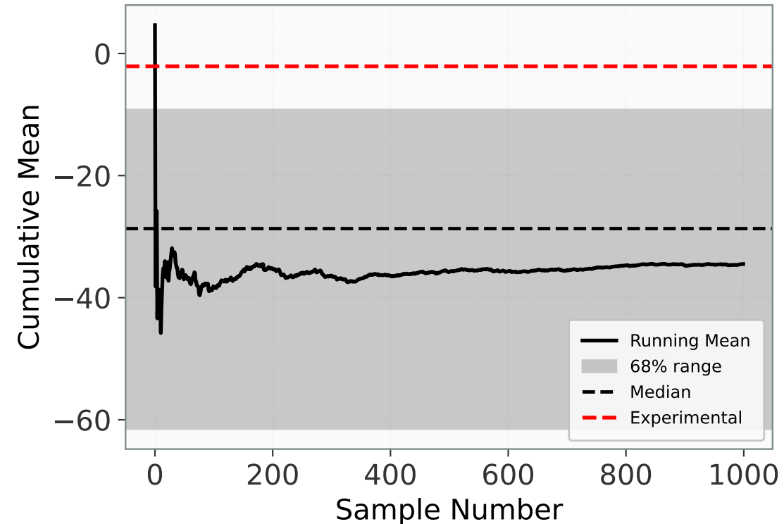
Convergence: \xi_{180,60}
