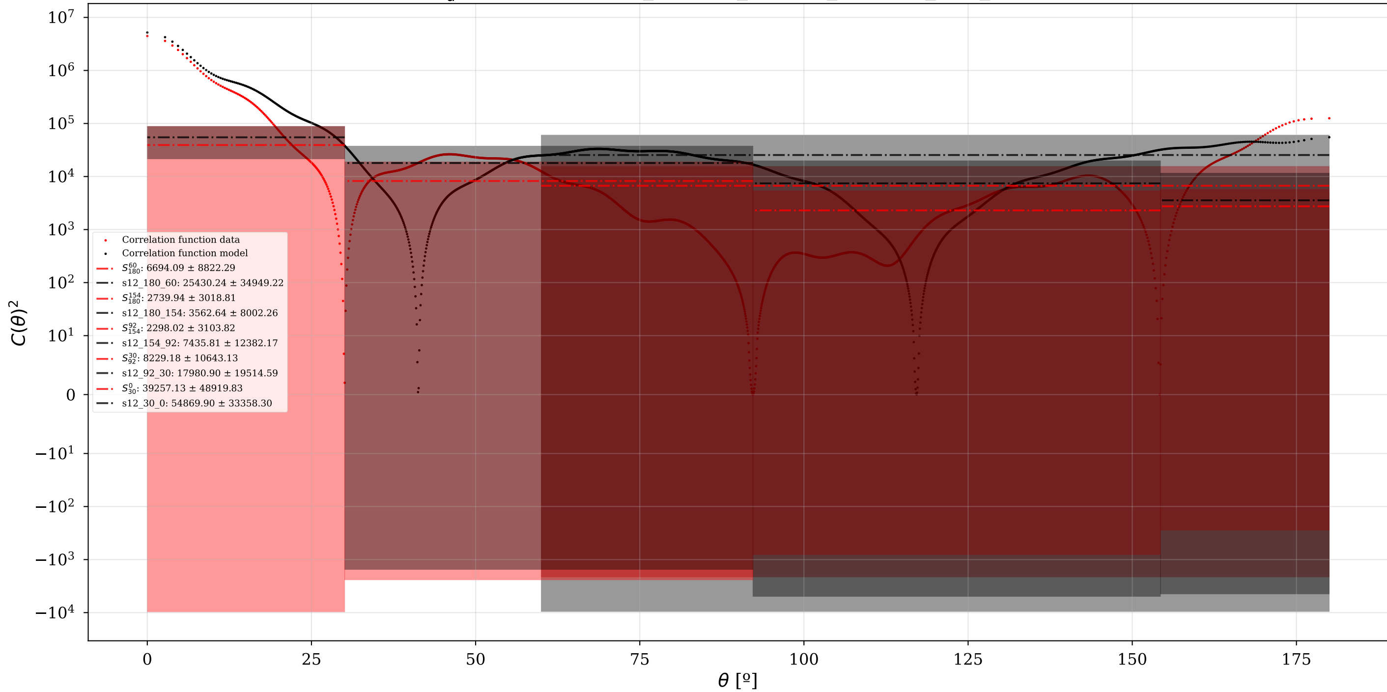
S_a^b analysis for base_omgak_plikHM_TTTEEE_lowl_lowE
