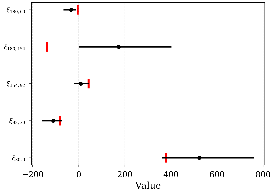
68% Credible Intervals
