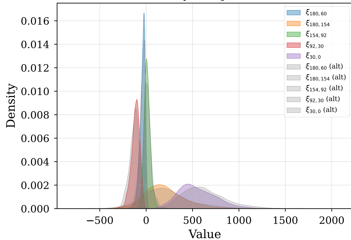
Density Comparison
