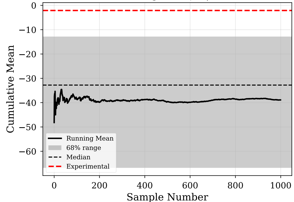
Convergence: \xi_{180,60}
