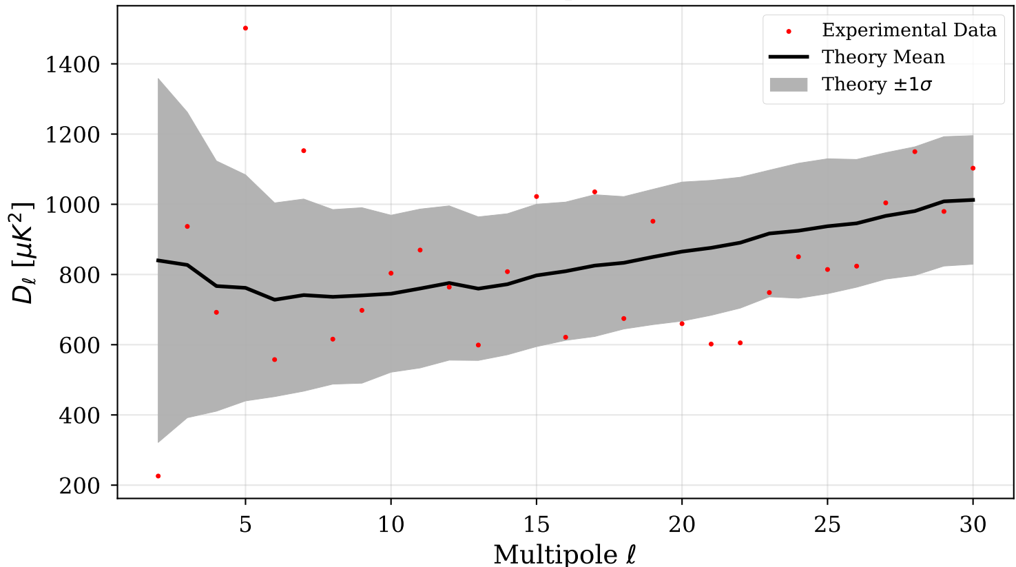
Power Spectrum
