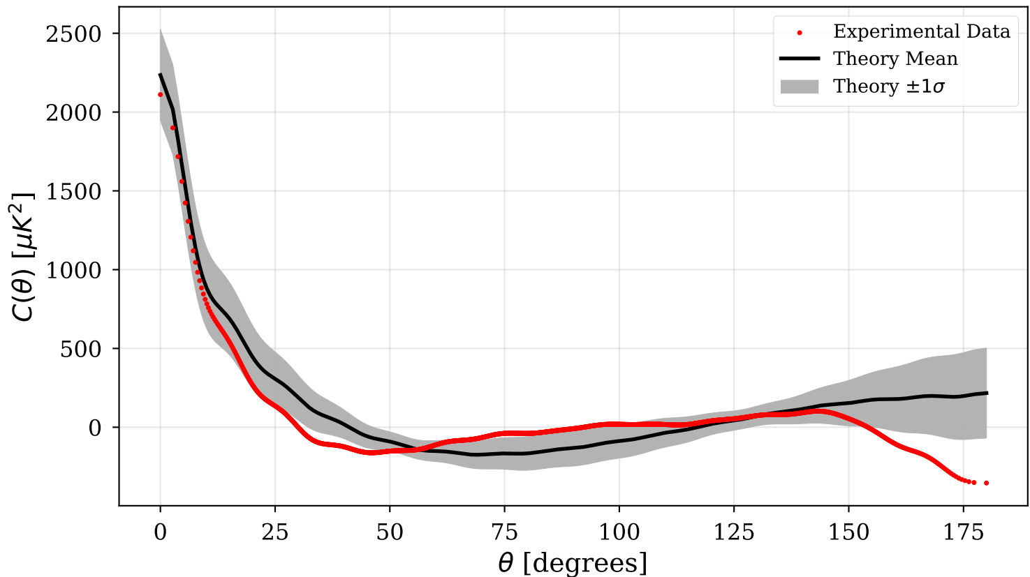
Correlation Function
