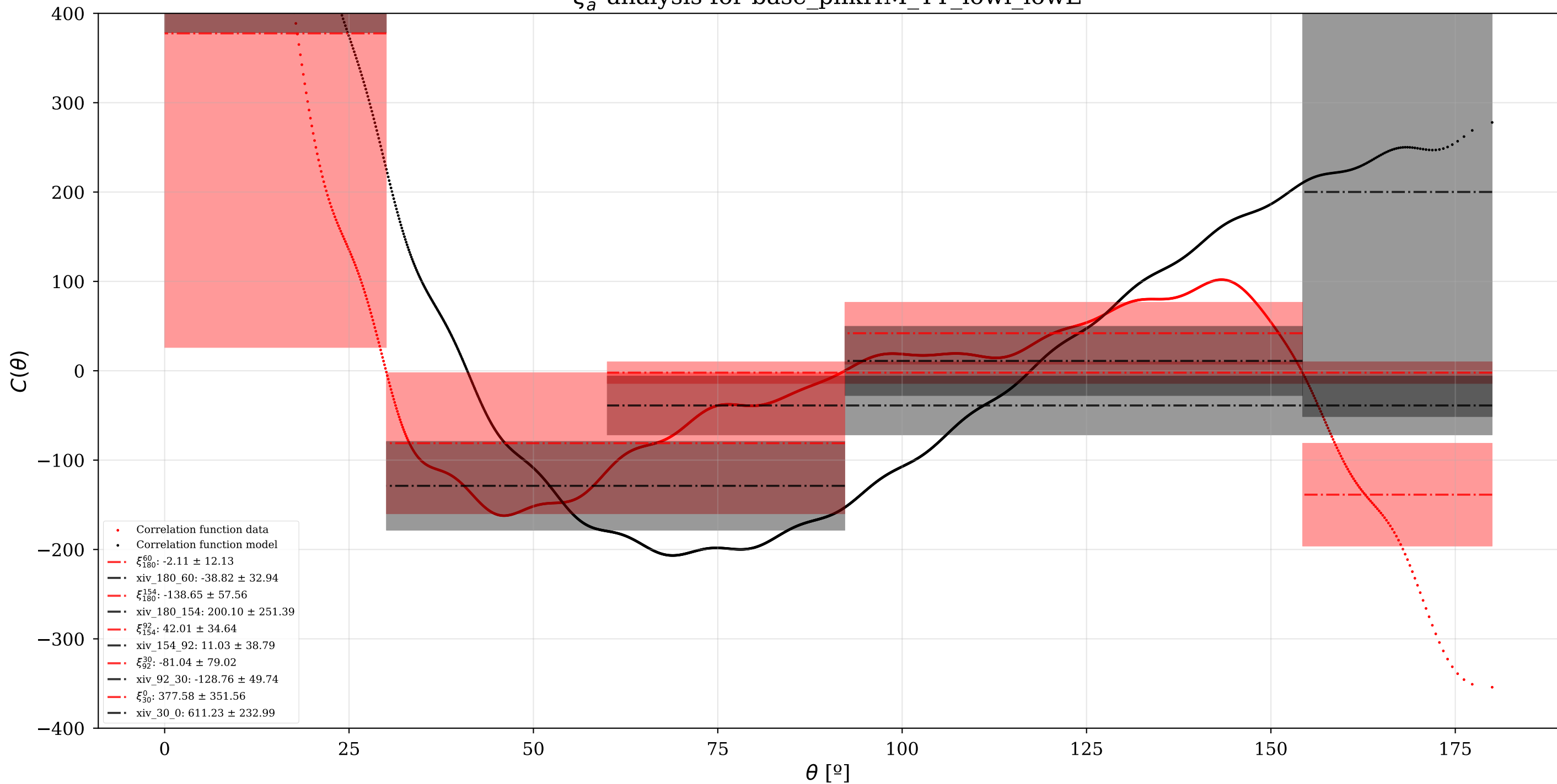
\xi_a^b analysis for base_plikHM_TT_lowl_lowE
