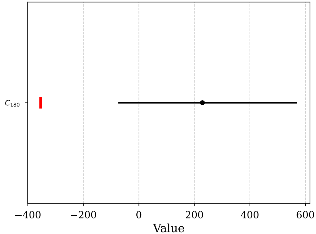
68% Credible Intervals
