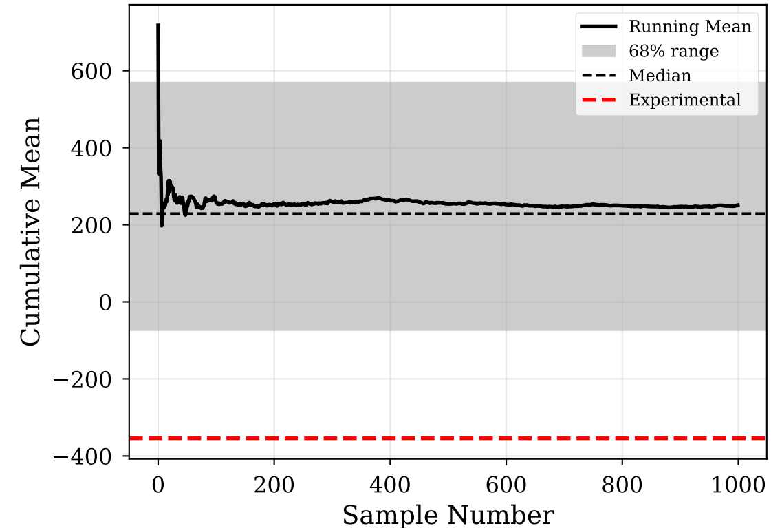
Convergence: C_{180}
