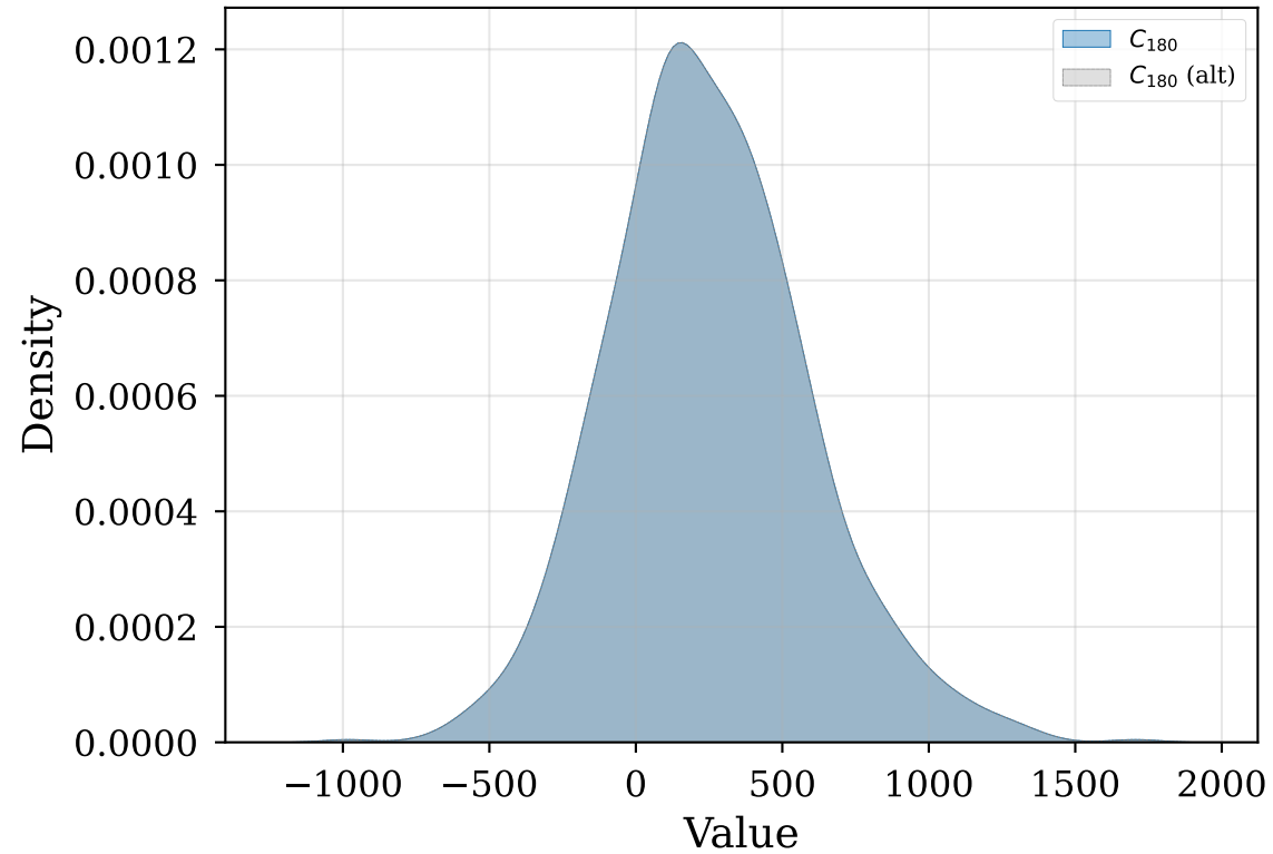
Density Comparison
