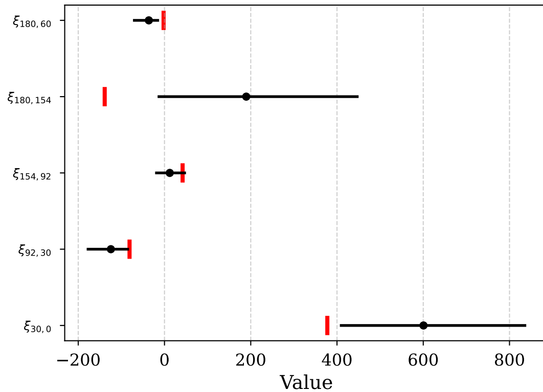
68% Credible Intervals
