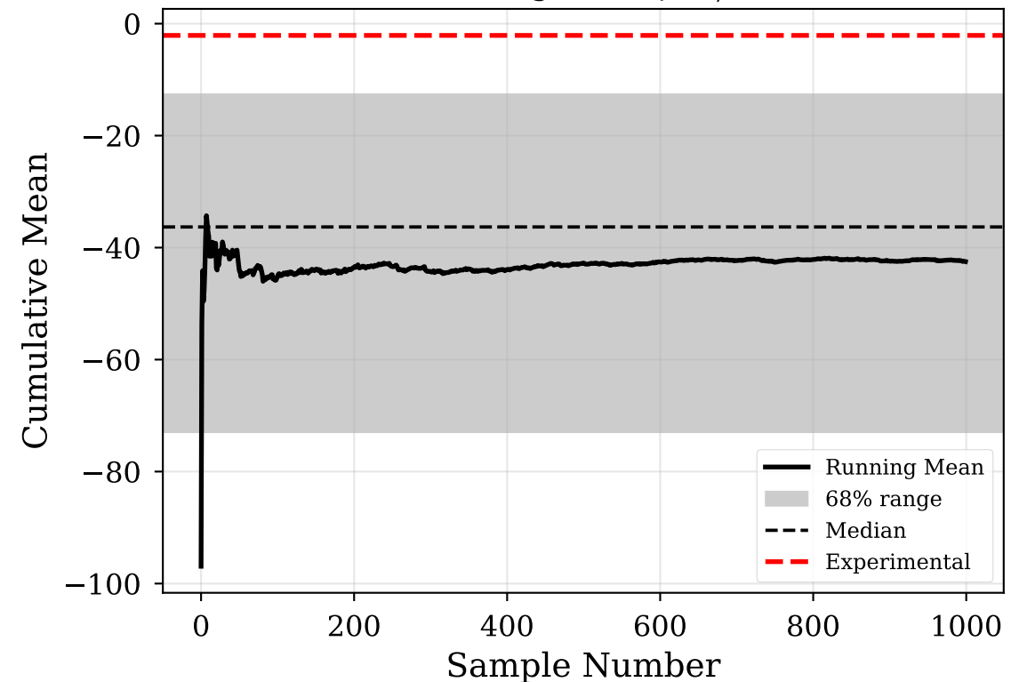
Convergence: \xi_{180,60}
