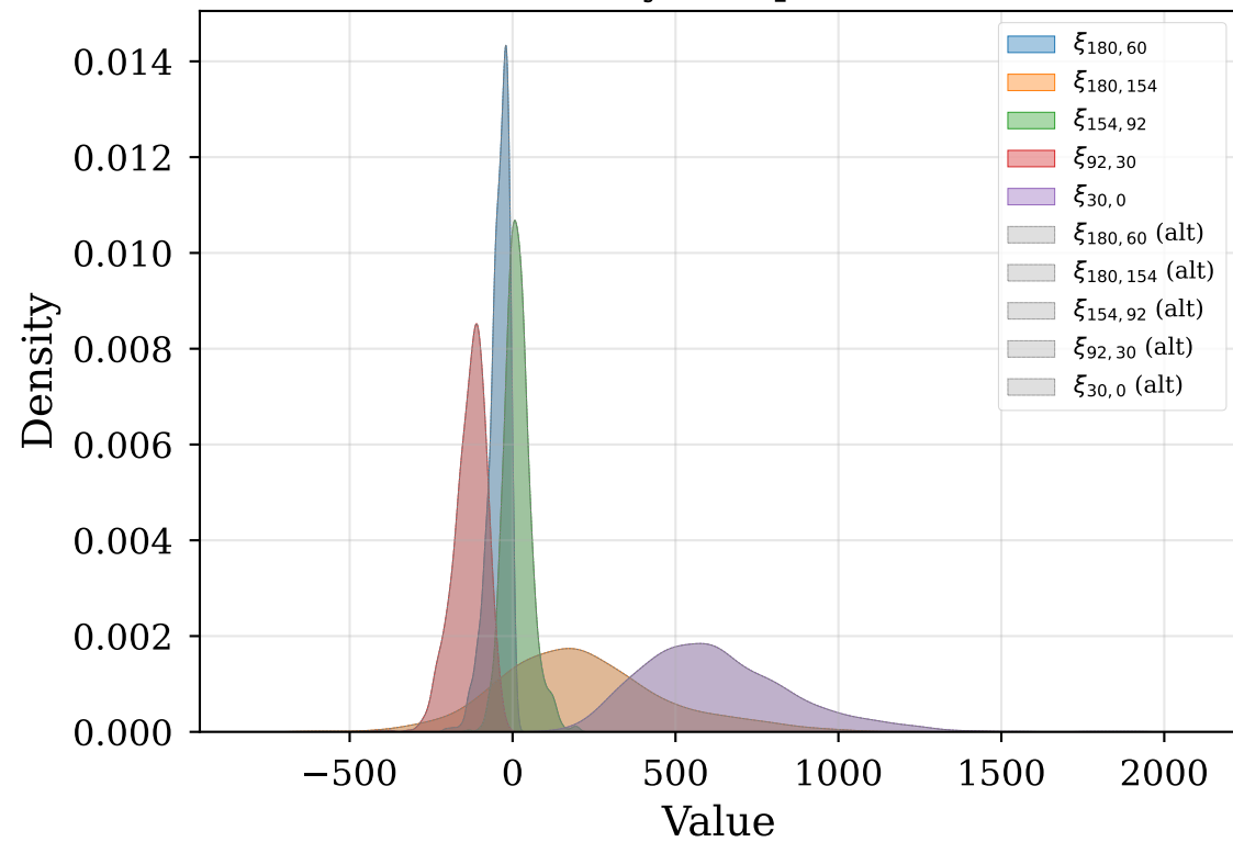
Density Comparison
