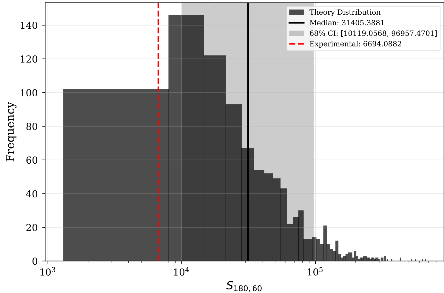
Distribution: S_{180,60} p-val = 0.075
