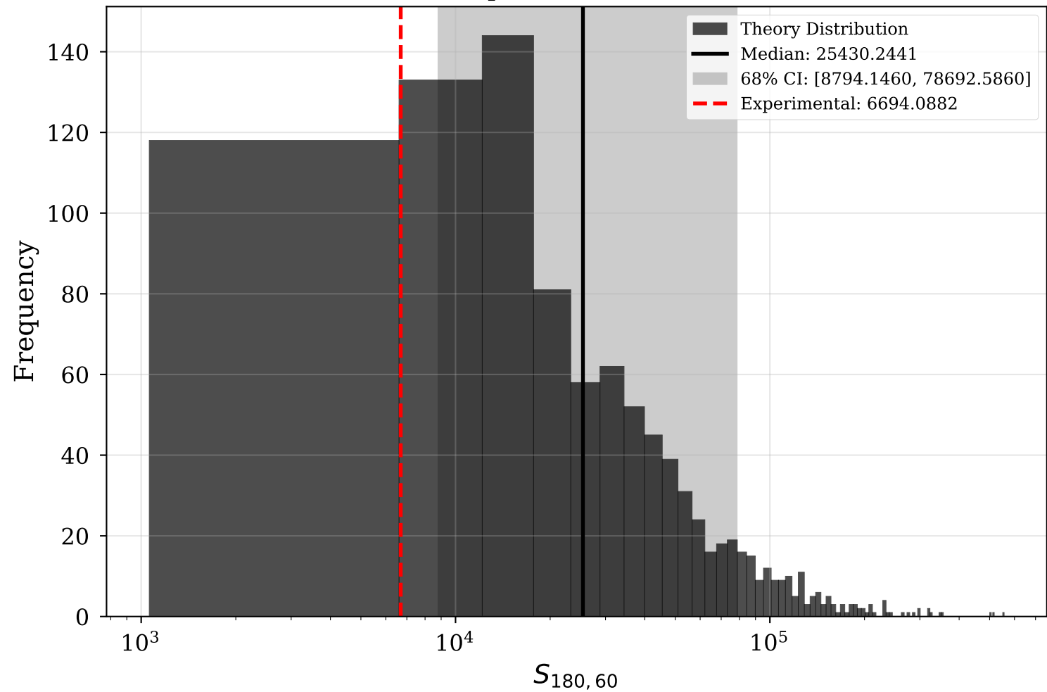
Distribution: S_{180,60} p-val = 0.119
