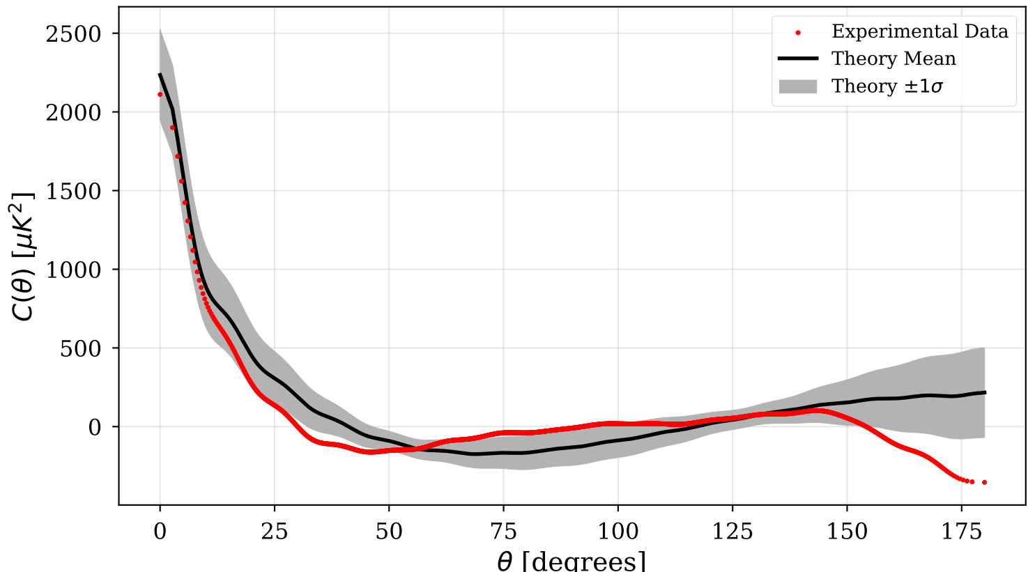
Correlation Function
