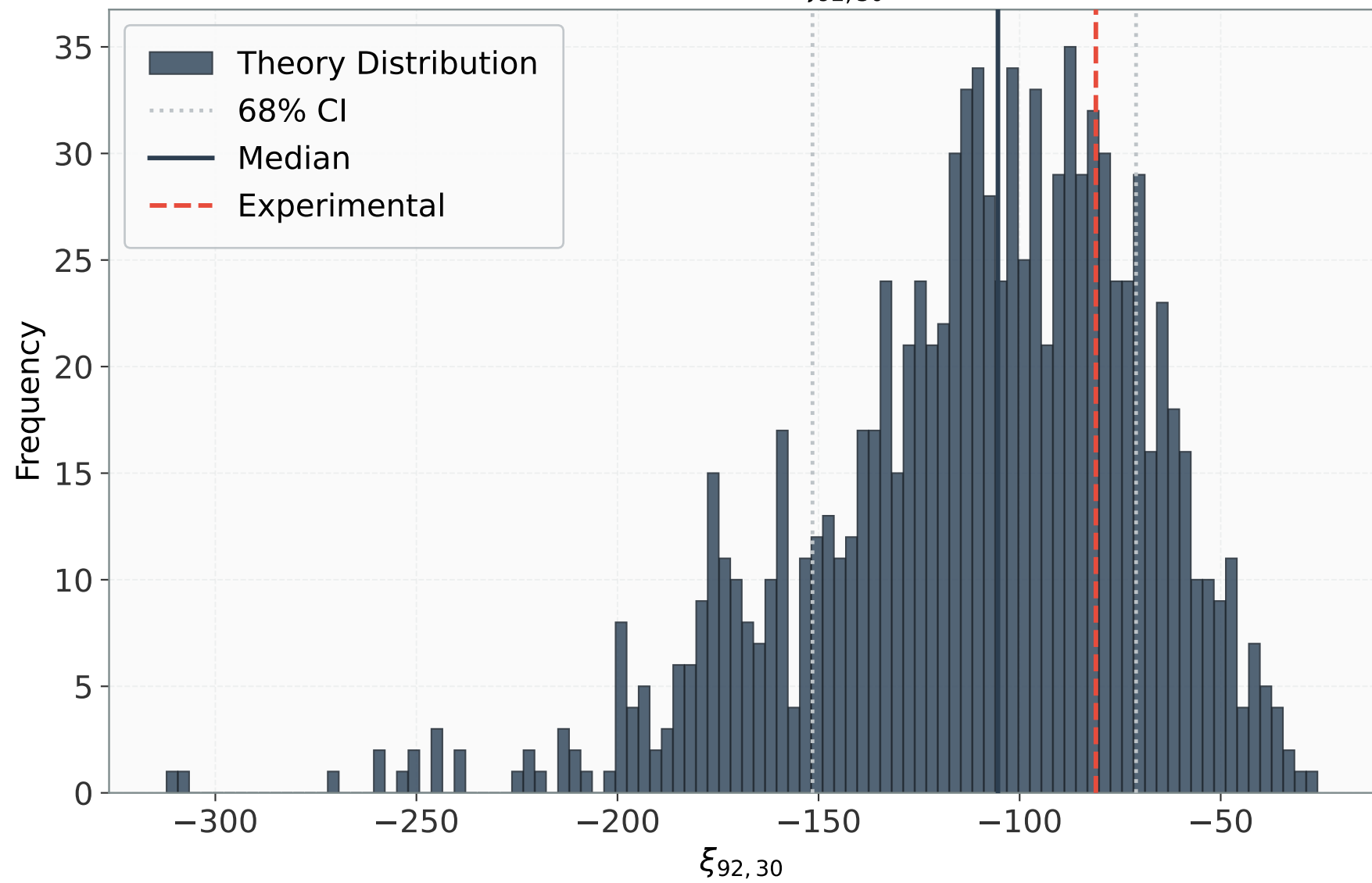
Distribution: \xi_{92,30}
