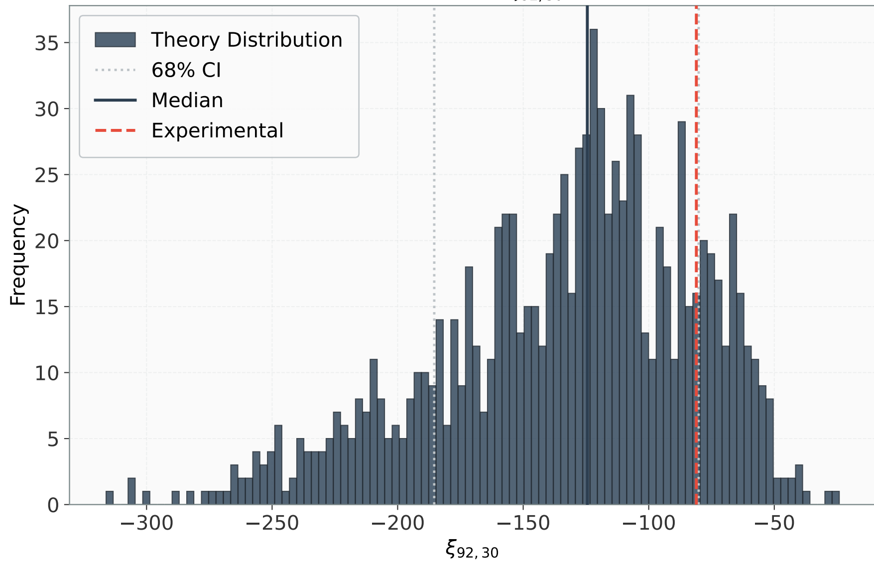
Distribution: \xi_{92, 30}
