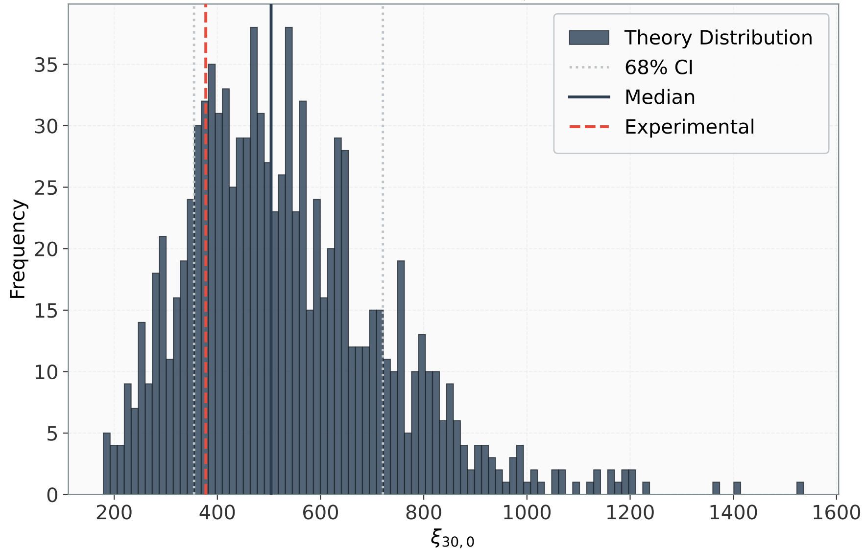
Distribution: \xi_{30,0}
