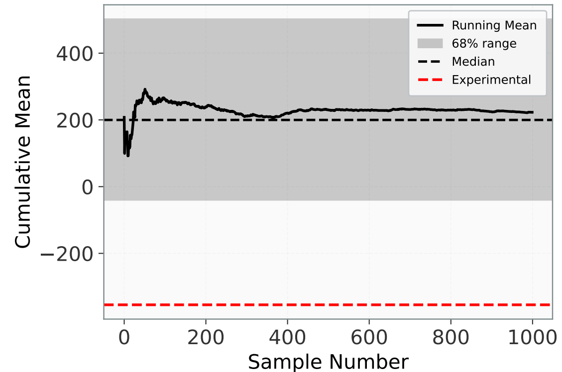
Convergence: C_{180}
