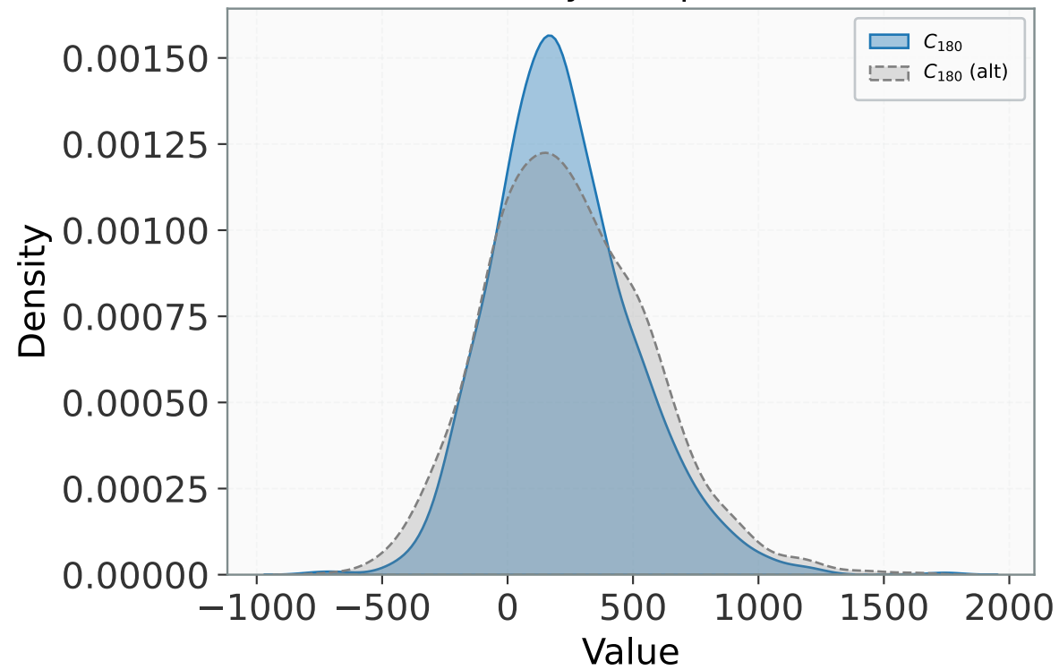
Density Comparison
