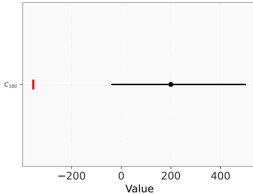
68% Credible Intervals
