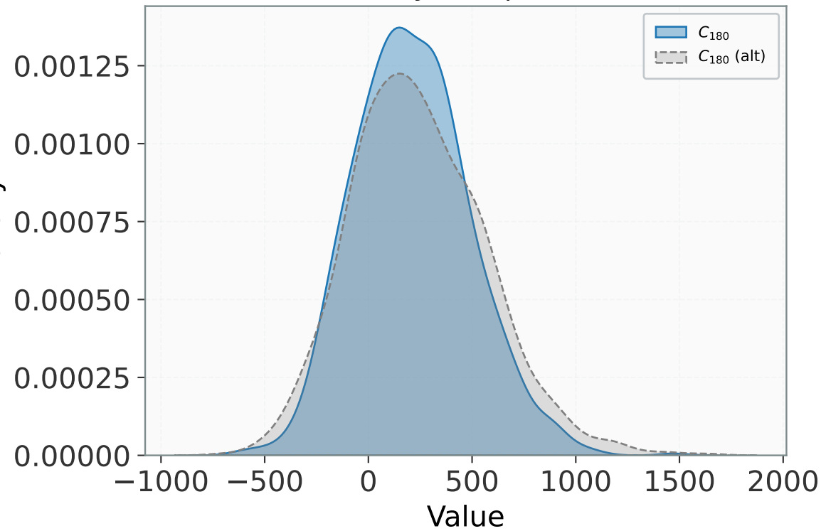
Density Comparison
