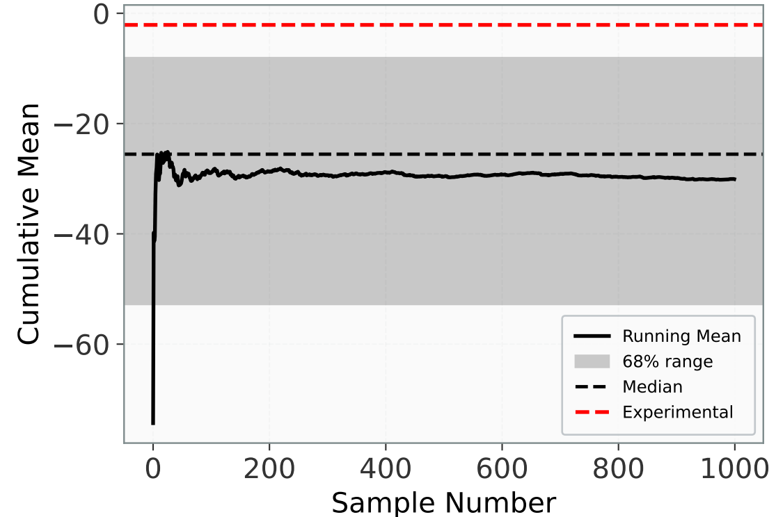
Convergence: \xi_{180,60}
