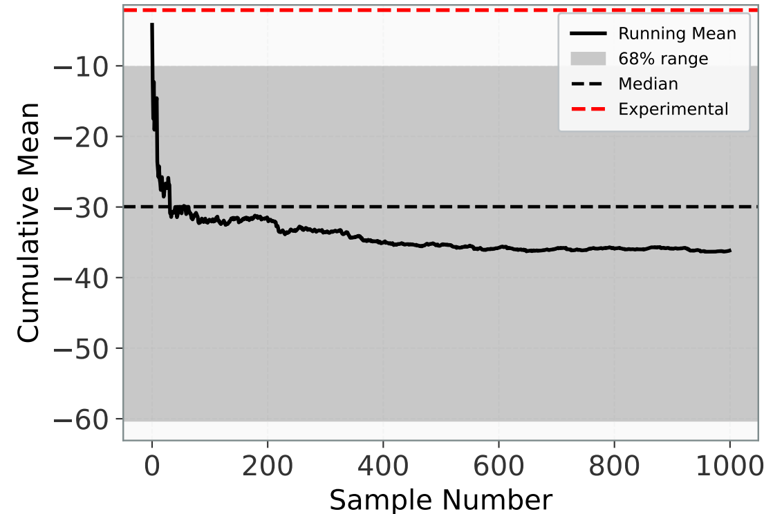
Convergence: \xi_{180,60}
