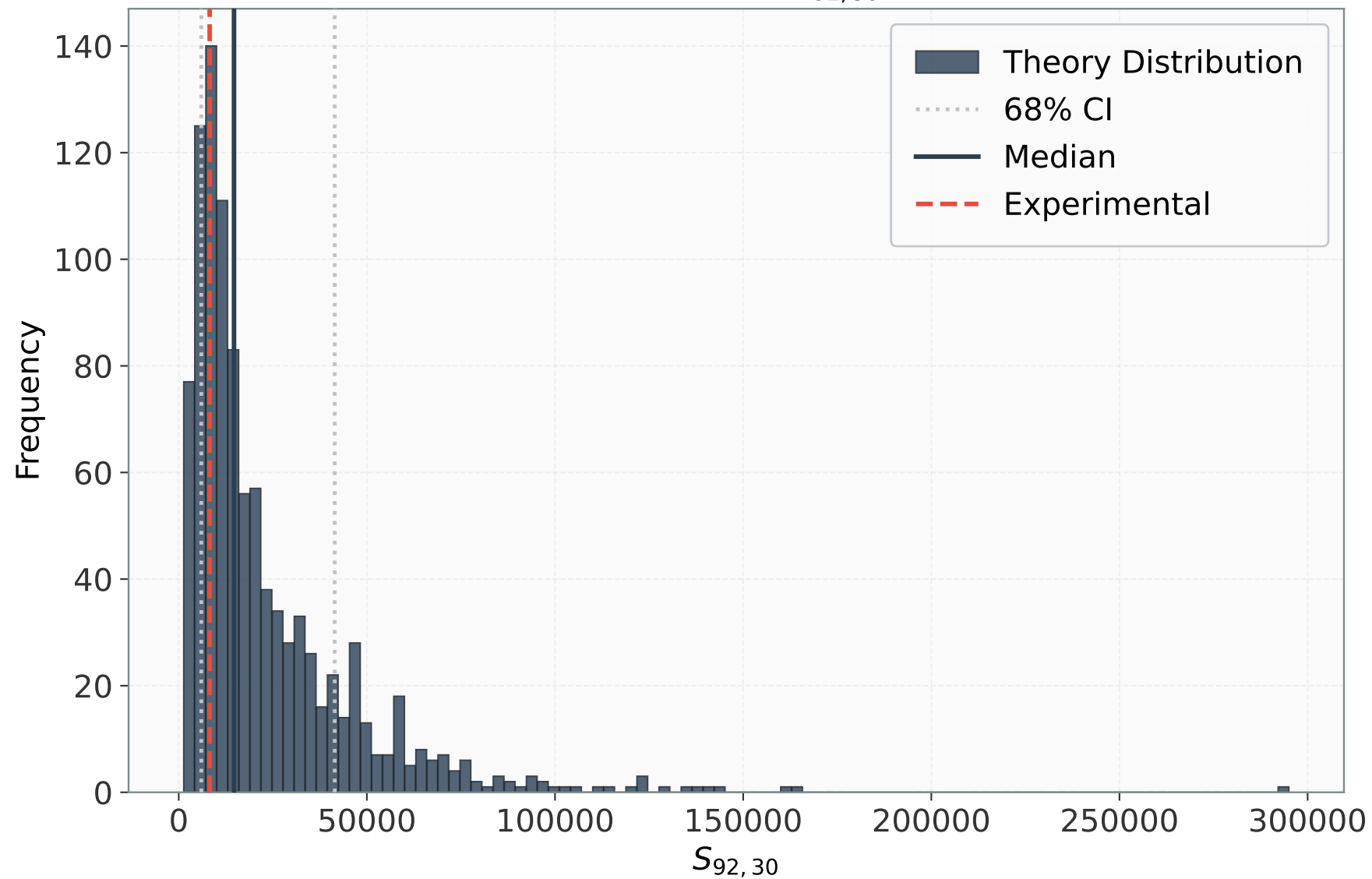
Distribution: S_{92,30}
