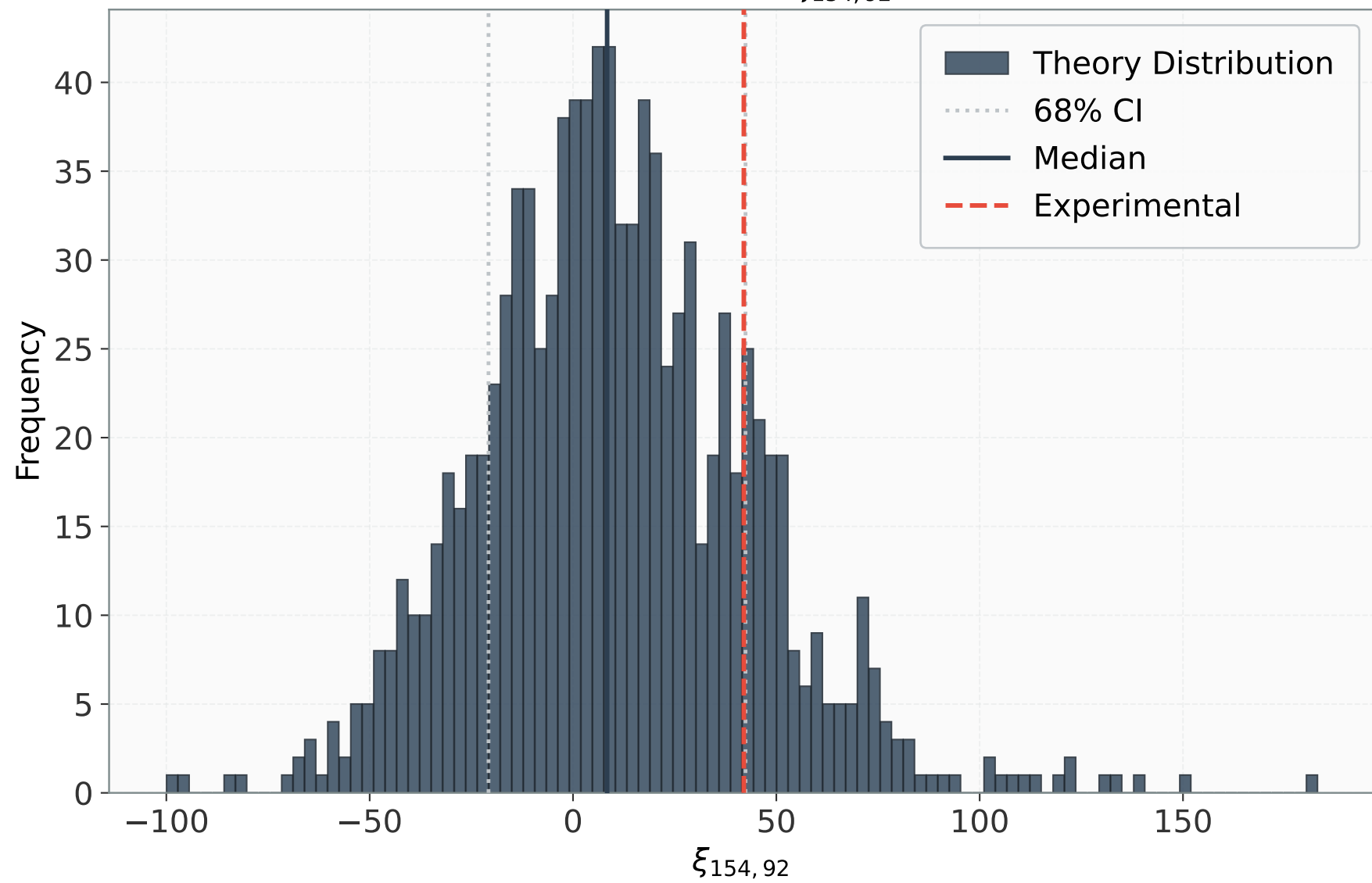
Distribution: \xi_{154,92}
