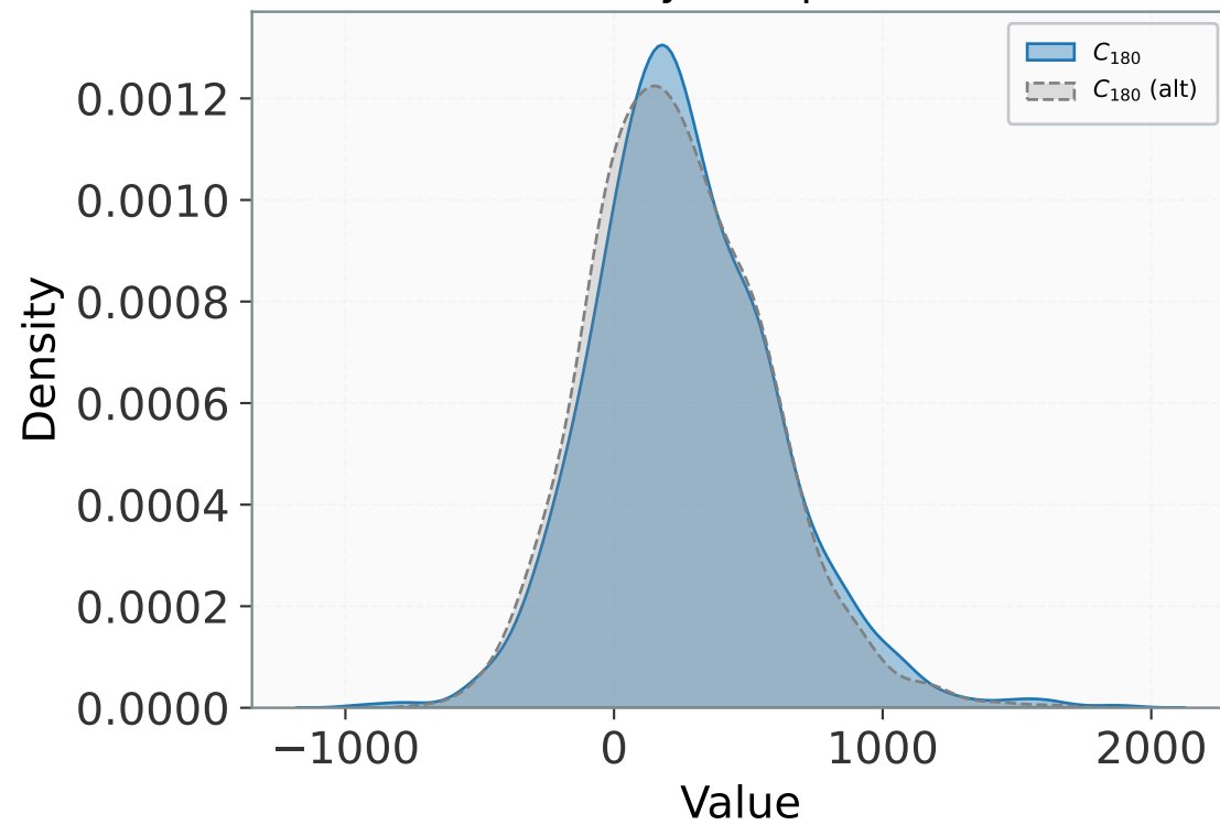
Density Comparison
