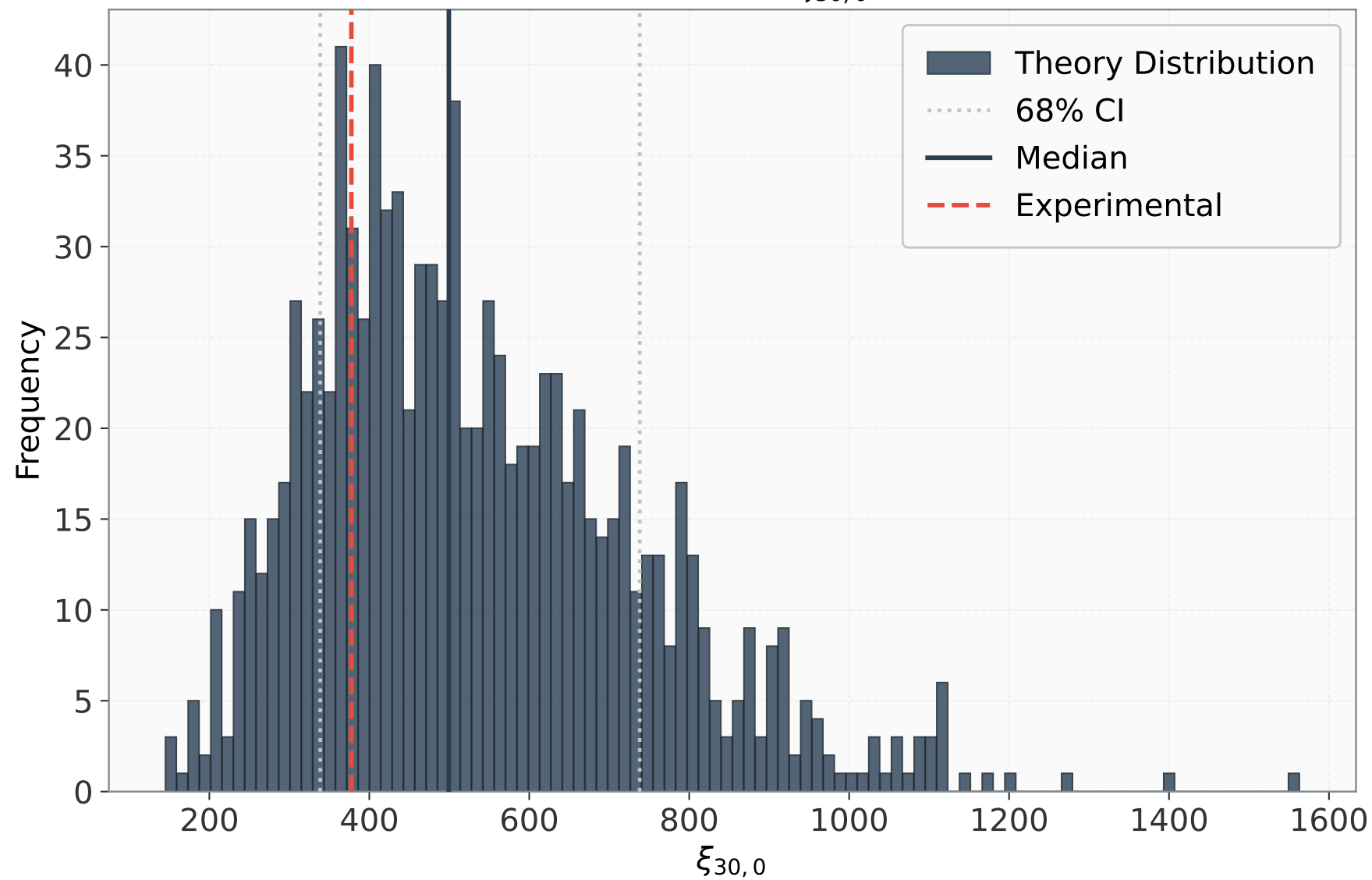
Distribution: \xi_{30,0}
