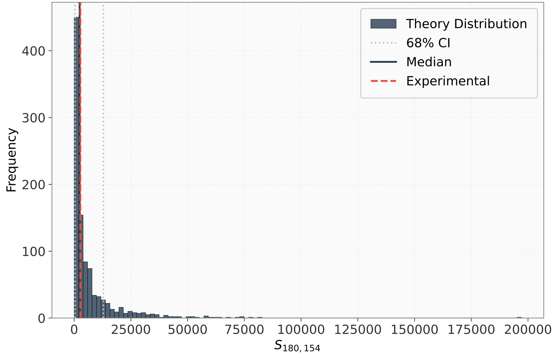
Distribution: S_{180,154}
