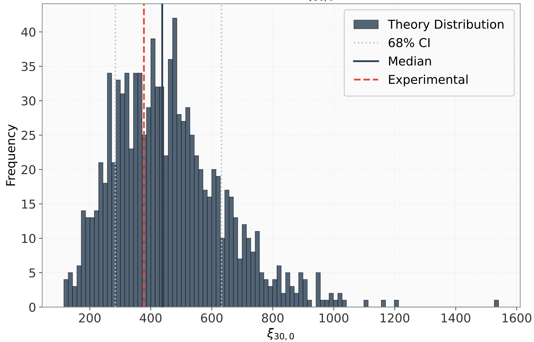
Distribution: \xi_{30,0}
