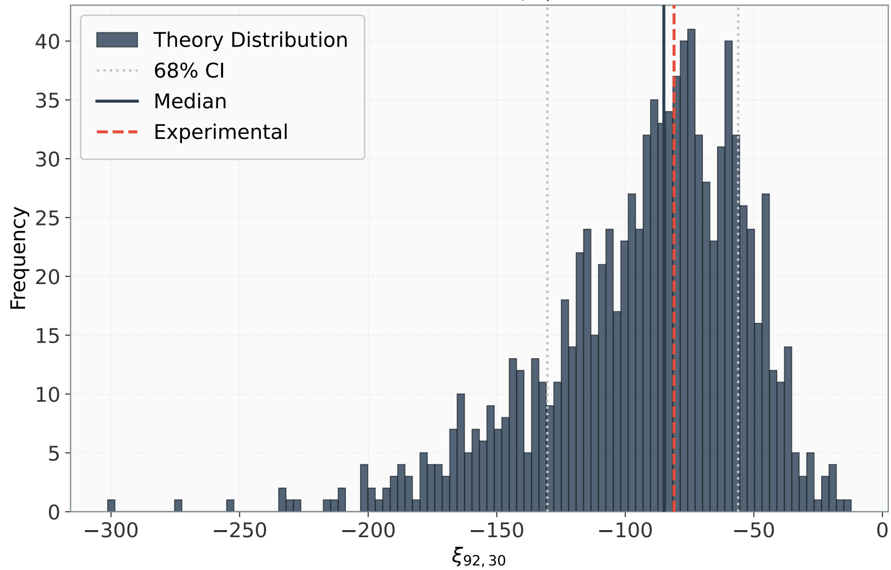
Distribution: \xi_{92,30}
