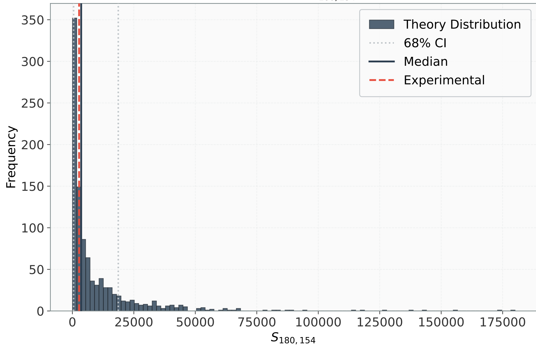
Distribution: S_{180,154}
