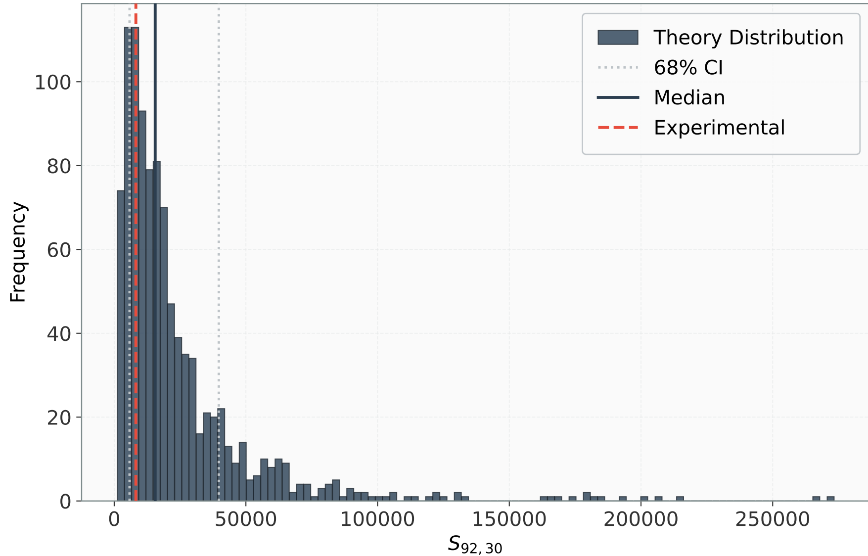
Distribution: S_{92,30}
