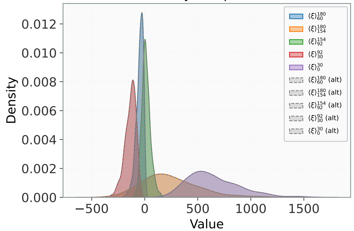
Density Comparison
