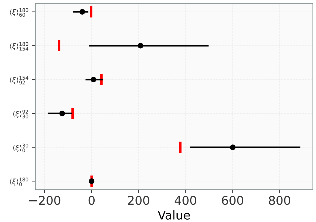
68% Credible Intervals
