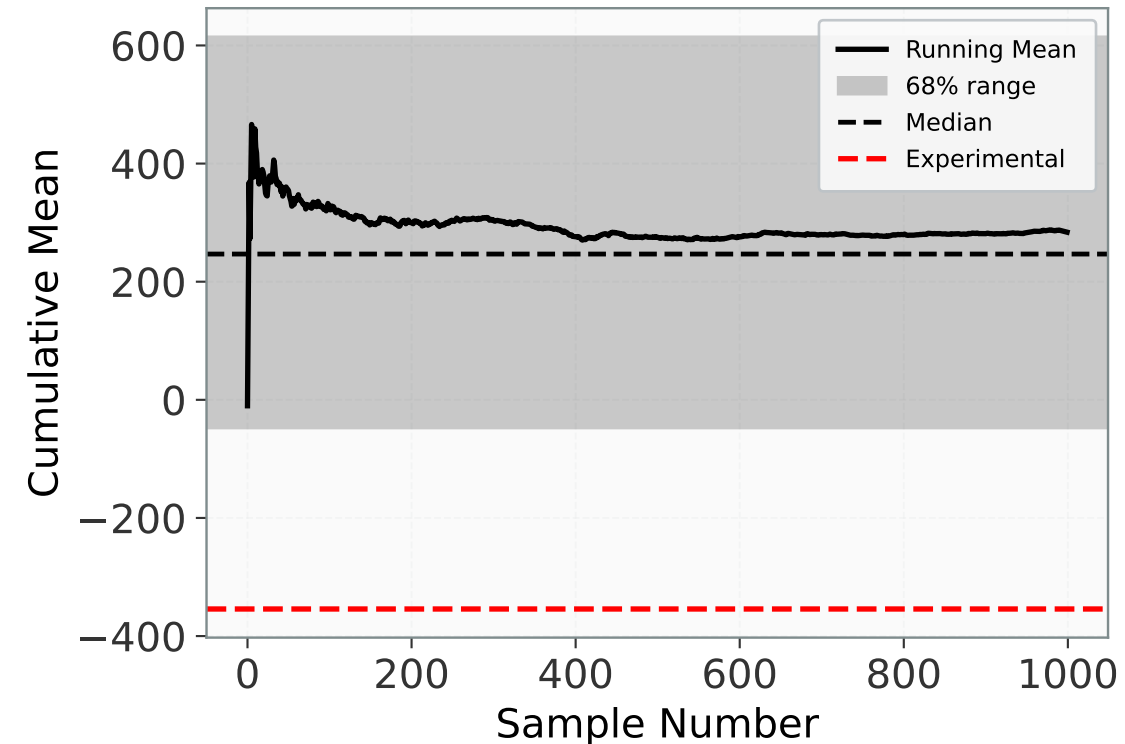
Convergence: \xi_{180}
