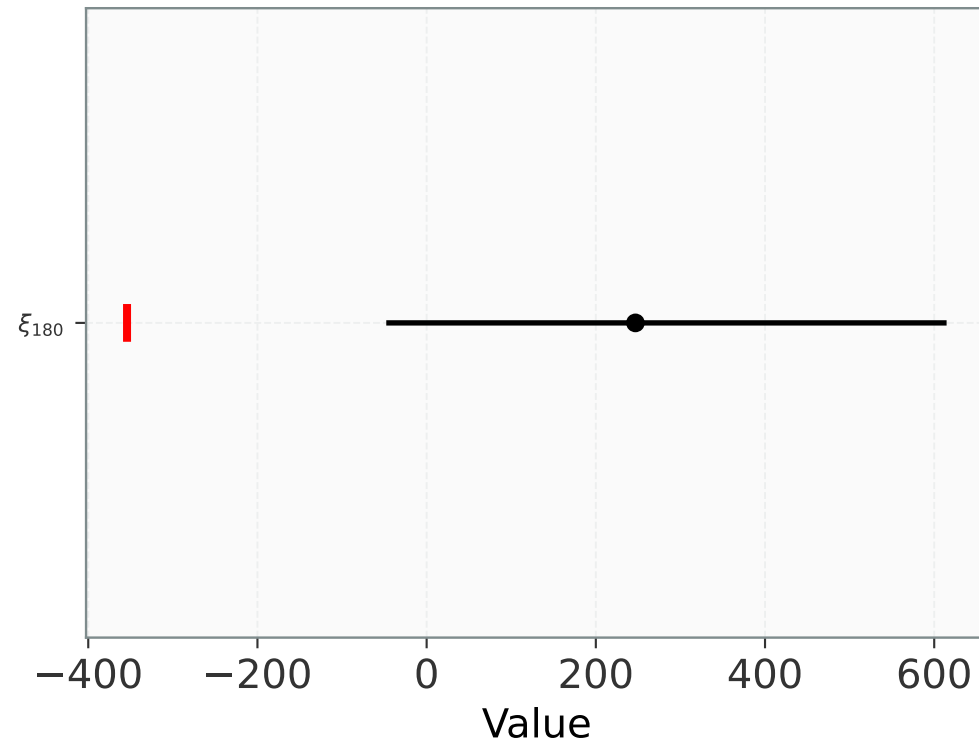
68% Credible Intervals
