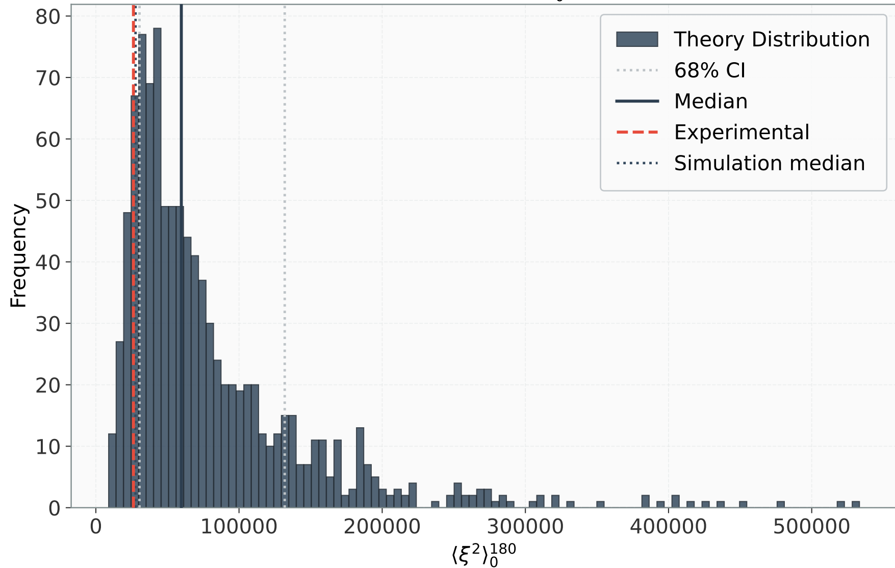
Distribution: \langle \xi^2 \rangle_0^{180}
